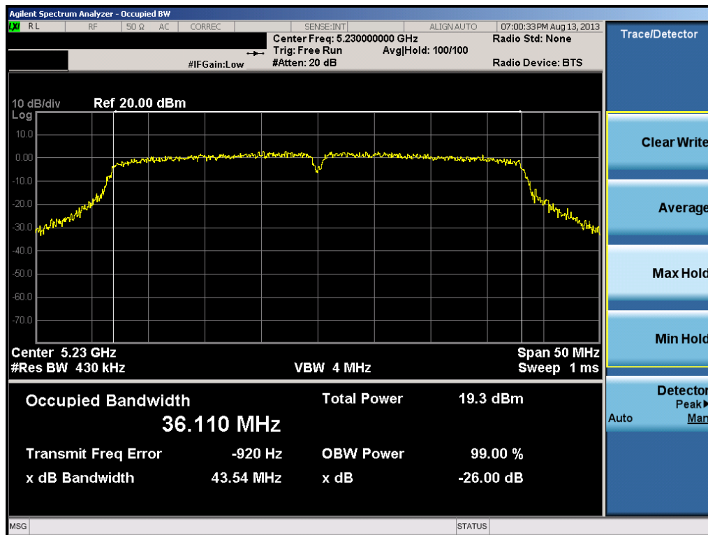
Plot 6-8. 26dB Bandwidth Plot (40MHz BW 802.11a/n (UNII Band 1) – Ch. 46)
