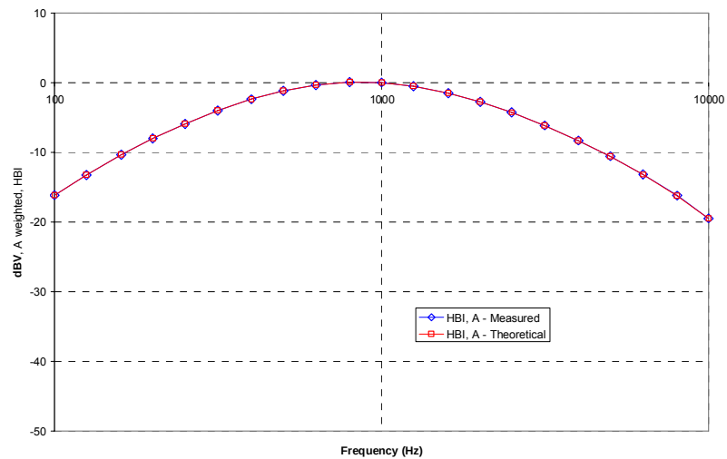
Figure 5-8 ABM2 Frequency Response Validation
