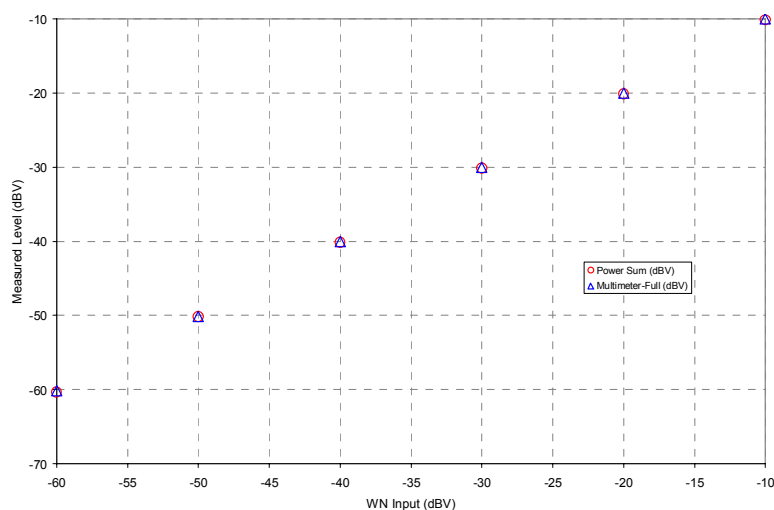
Figure 5-10 ABM2 Power Sum Validation
