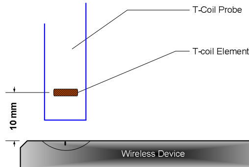
Figure 5-11 Measurement Distance
