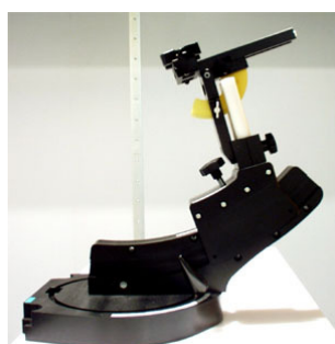
Figure 3.8 Device Holder
