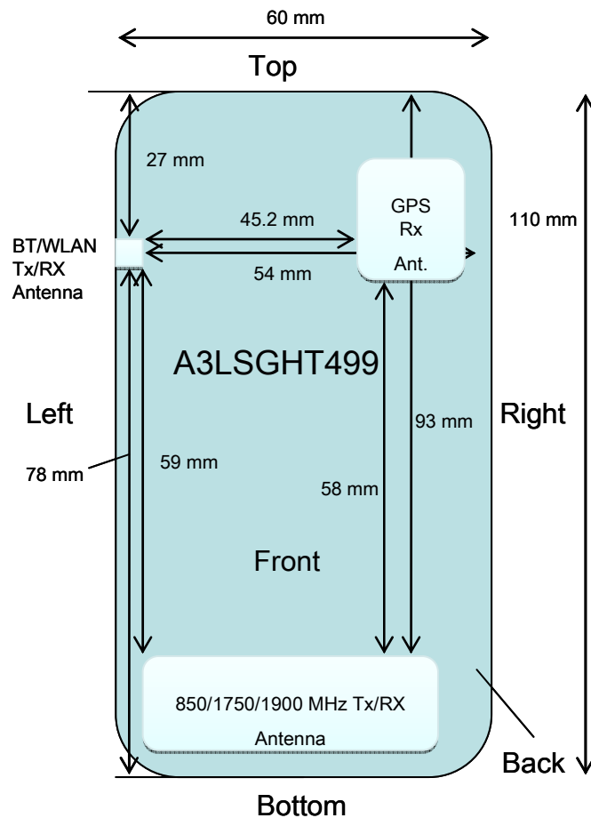
Figure 13-1 Identification of Sides for SAR Testing
