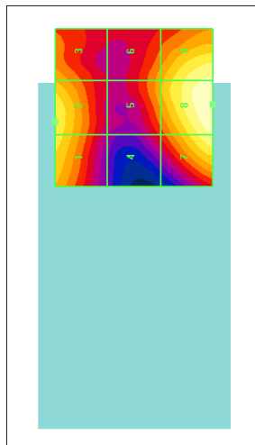
Figure 10-1 Sample E-field Scan Overlay (See Test Setup Photographs for actual WD overlay)
