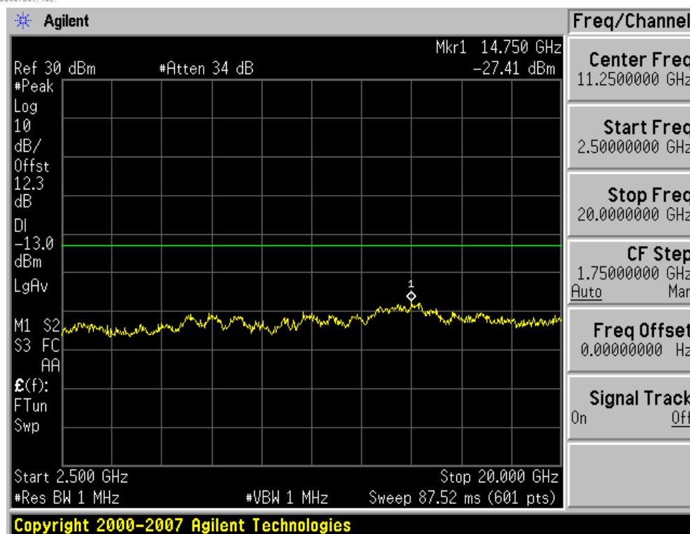
Plot 7-15. Conducted Spurious Plot (PCS GSM Mode – Ch. 661)
