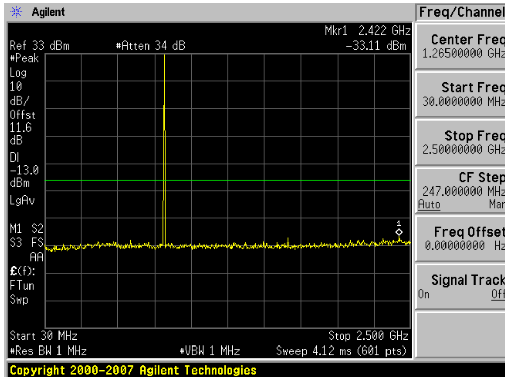
Plot 7-4. Conducted Spurious (Cellular GSM Mode – Ch. 190)
