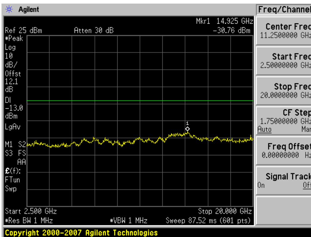
Plot 7-24. Conducted Spurious Plot (AWS WCDMA Mode – Ch. 1312)
