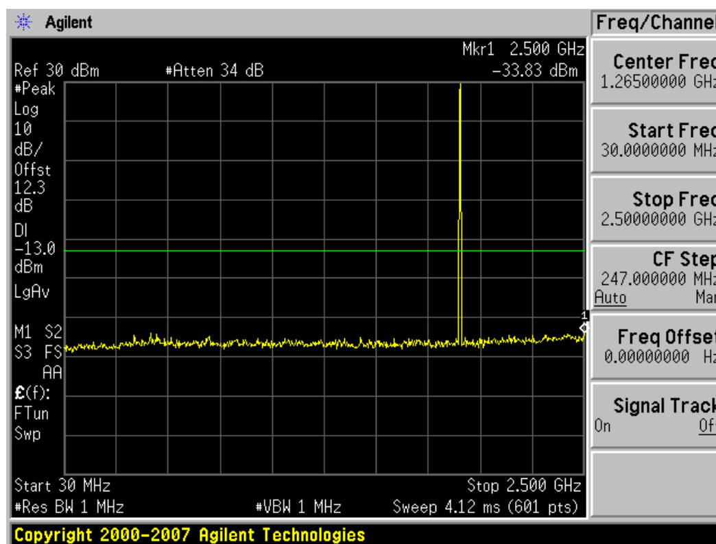
Plot 7-18. Conducted Spurious Plot (PCS GSM Mode – Ch. 810)
