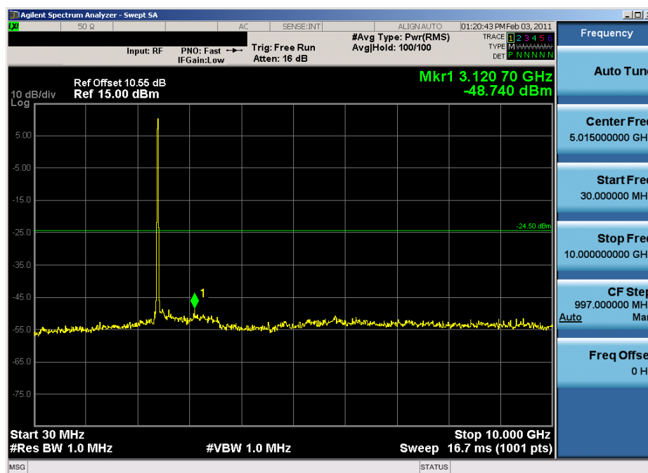
Plot 6-25. Conducted Spurious Plot (802.11b – Ch. 1)
