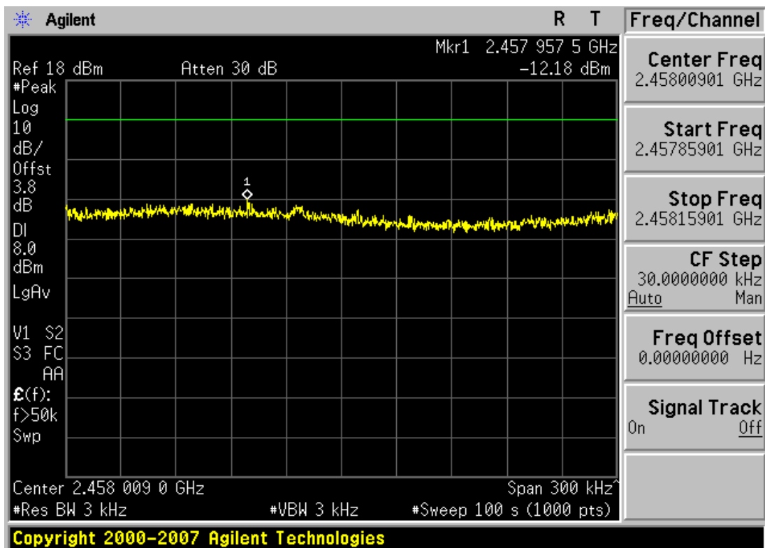
Plot 6-12. Power Spectral Density Plot (802.11g – Ch. 11)
