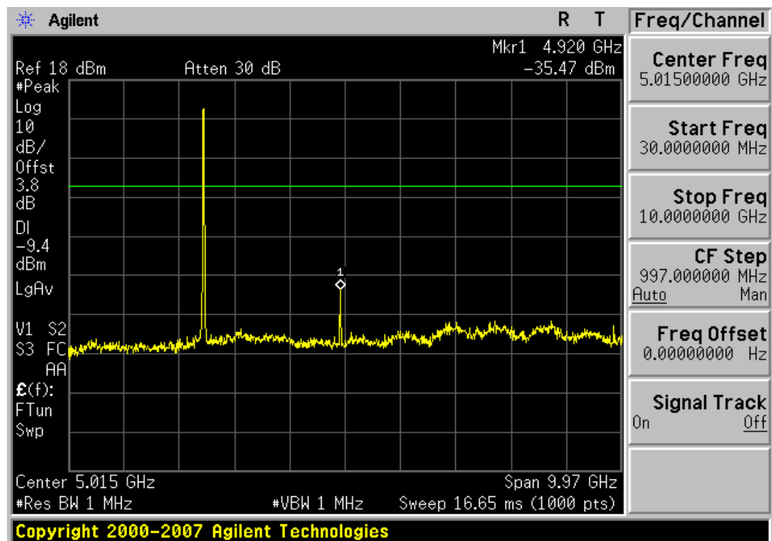
Plot 6-21. Conducted Spurious Plot (802.11b – Ch. 11)
