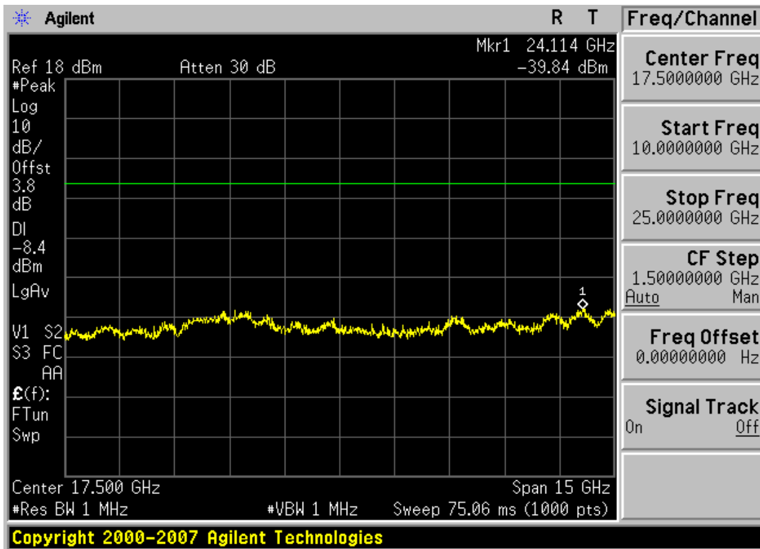
Plot 6-18. Conducted Spurious Plot (802.11b – Ch. 1)
