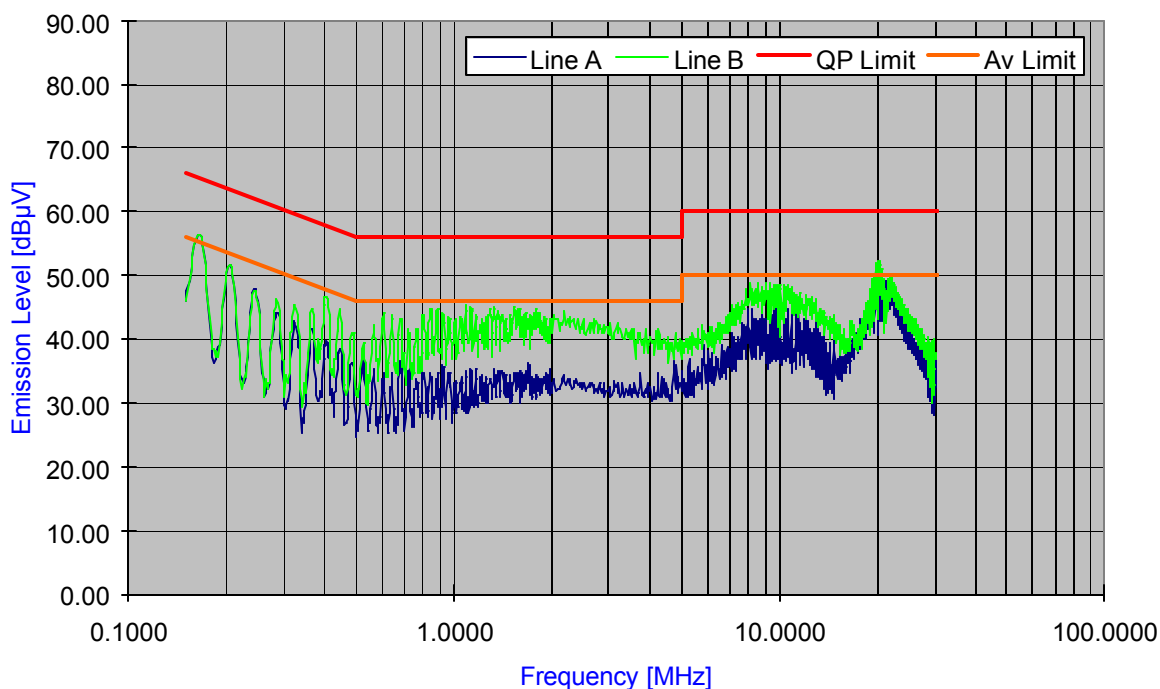
Plot 6-24. Line Conducted Plot with 802.11g
