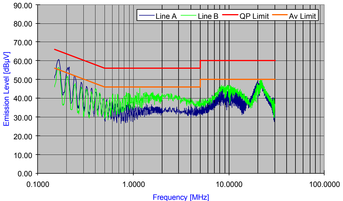
Plot 6-23. Line Conducted Plot with 802.11b
