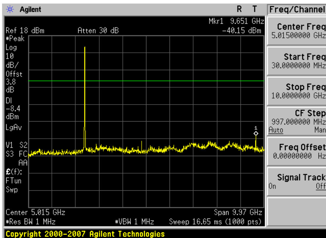
Plot 6-17. Conducted Spurious Plot (802.11b – Ch. 1)
