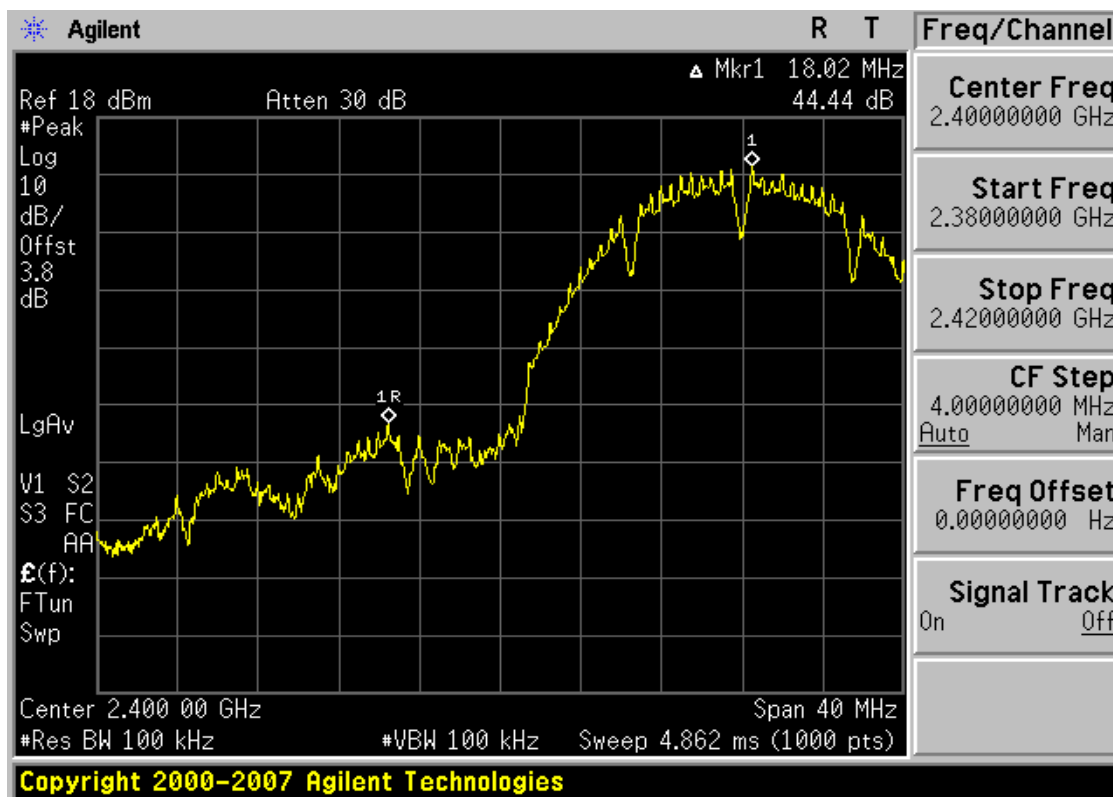
Plot 6-13. Band Edge Plot (802.11b – Ch. 1)
