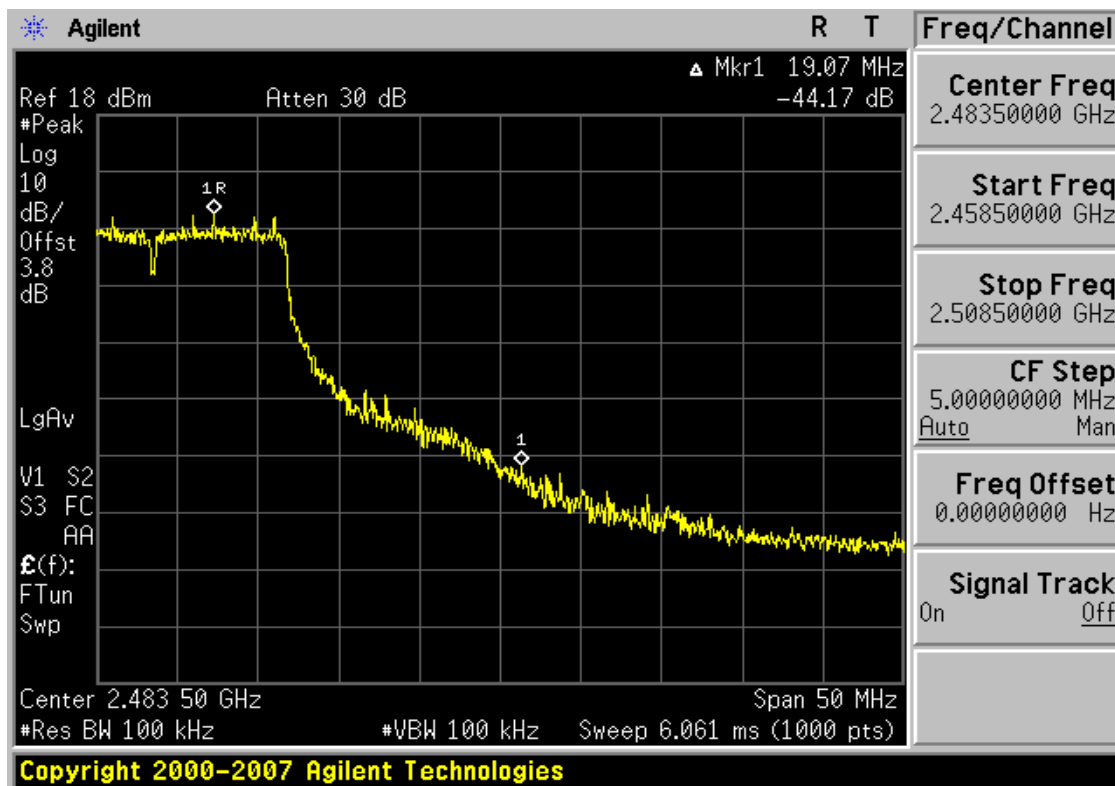
Plot 6-16. Band Edge Plot (802.11g – Ch. 11)
