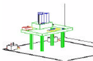
Figure 3-3. Wooden Table & Bonded LISNs
