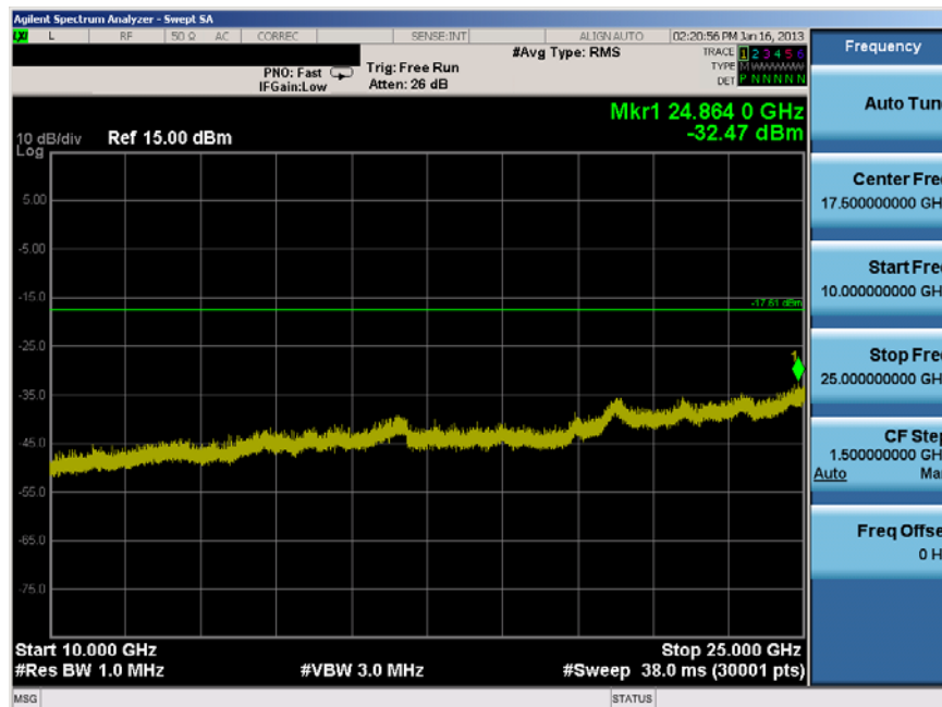
Plot 6-37. Conducted Spurious Plot (Bluetooth, 1Mbps – Ch. 0)
