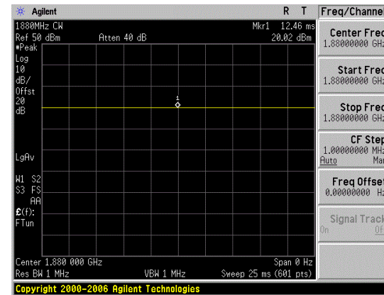
Figure 8.6 1880MHz CW Signal
