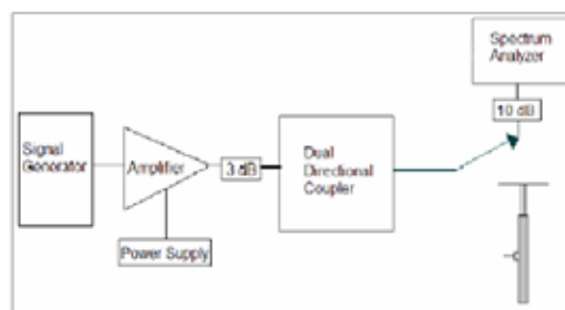
Figure 8.2 Setup to Peak Power using Spectrum Analyzer
