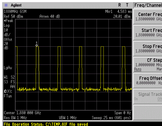
Figure 8.3 GSM1900 Signal
