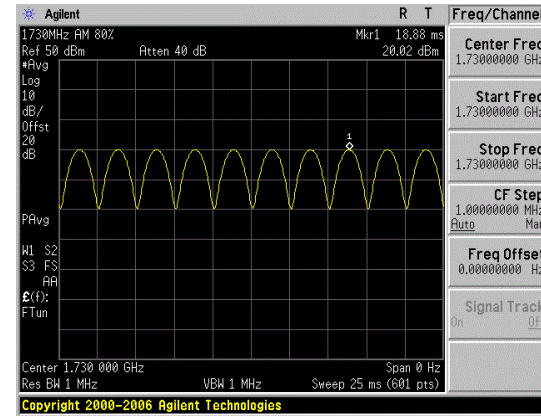
Figure 8.11 1730MHz 80% AM
