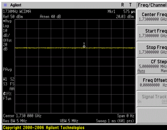
Figure 8.10 WCDMA1700 Signal
