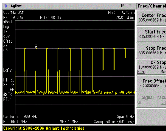
Figure 8.7 GSM850 Signal
