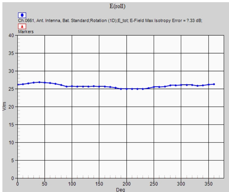
Peak Reading 360 degree Probe Rotation at Azimuth axis
