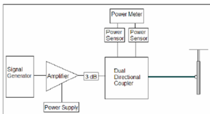
Figure 7.1 Dipole Validation Test Setup
