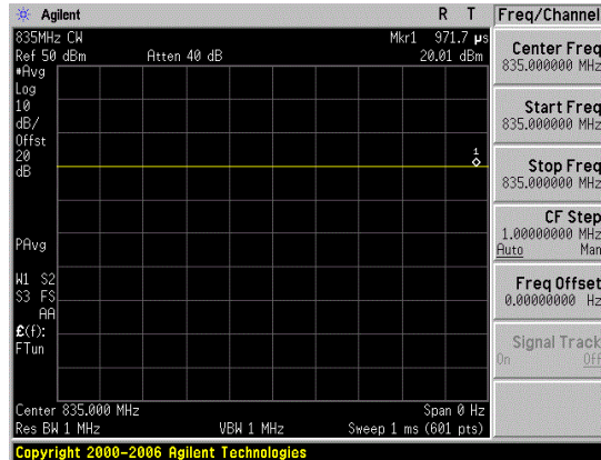
Figure 8.10 835MHz CW Signal
