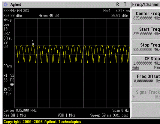
Figure 8.9 835MHz 80% AM Signal
