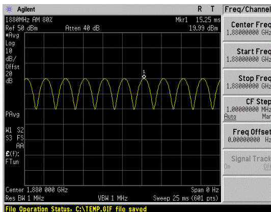
Figure 8.5 1880MHz 80% AM Signal
