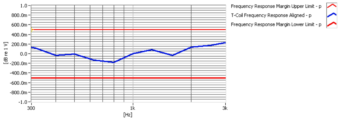
Figure 7-1 Helmholtz coil Validation for Frequency Response
