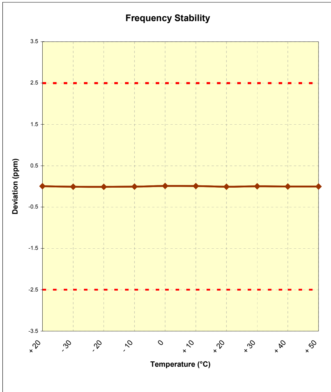
Figure 6-5. Frequency Stability Graph (AWS WCDMA Mode – Ch. 1412)
