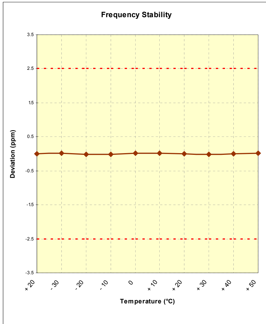
Figure 6-3. Frequency Stability Graph (Cell. WCDMA Mode – Ch. 4183)
