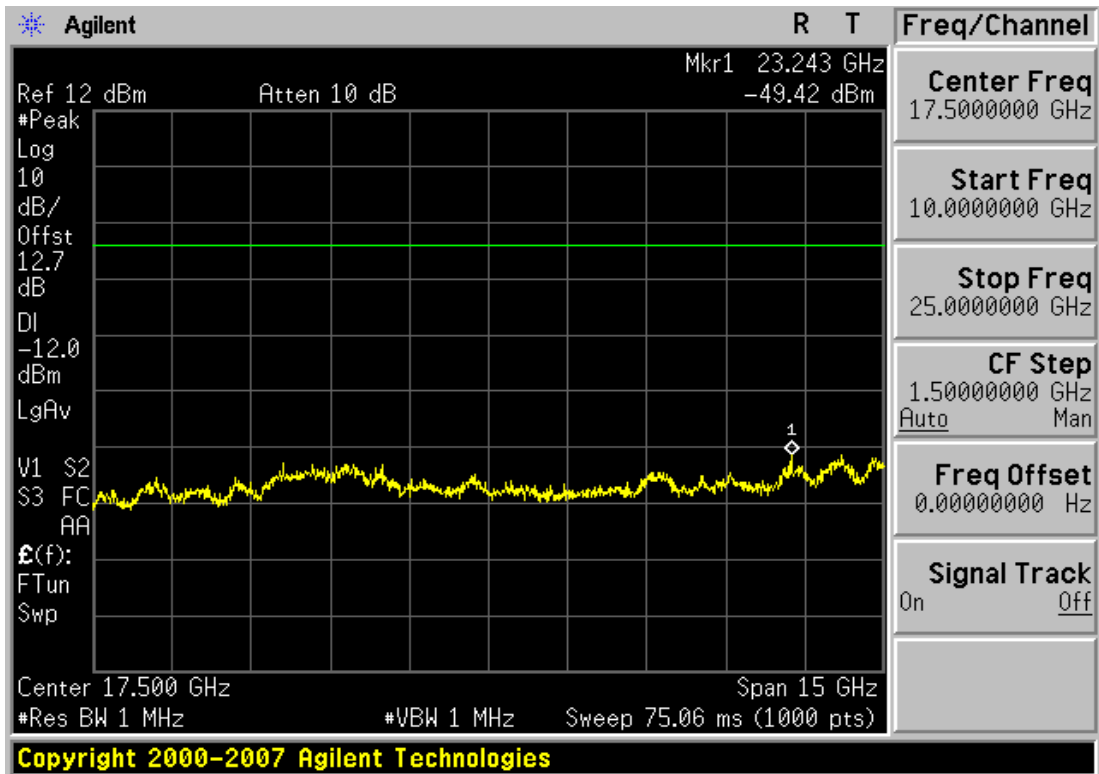
Plot 6-17. Conducted Spurious Plot (Bluetooth, 2Mbps - Ch. 0)
