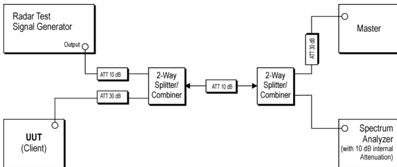
Figure 3-1. Conducted Test Setup for DFS
