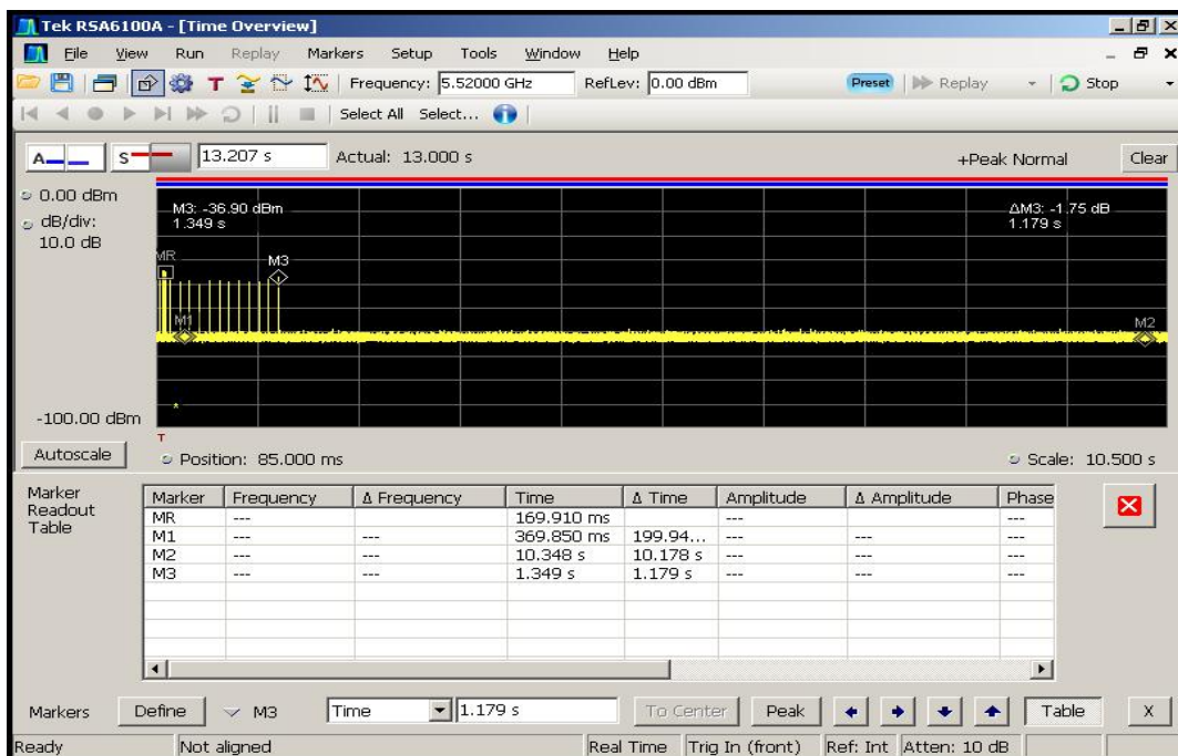
Figure 6-4. Channel Move Time (< 10sec)
