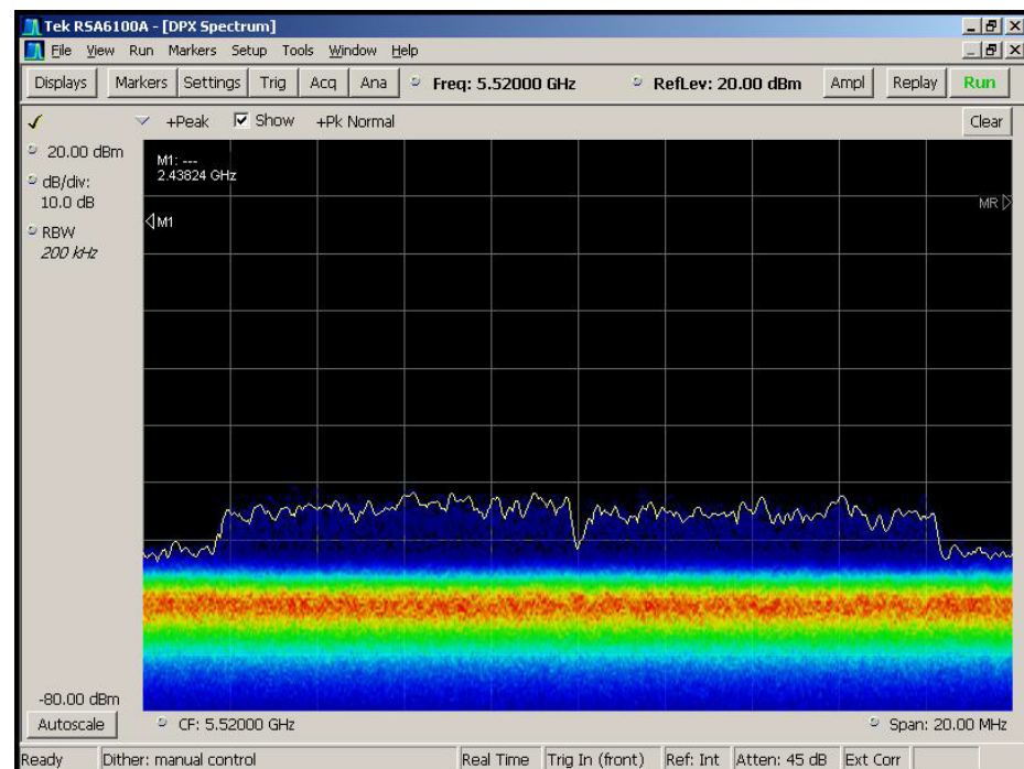
Figure 6-2. Real-Time Spectrum Display, No WLAN Traffic
