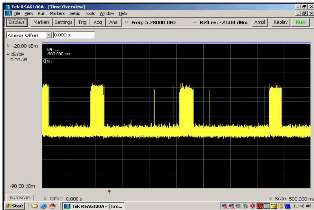
Figure 5-2. Time Display WLAN Channel Traffic (Streaming Video)
