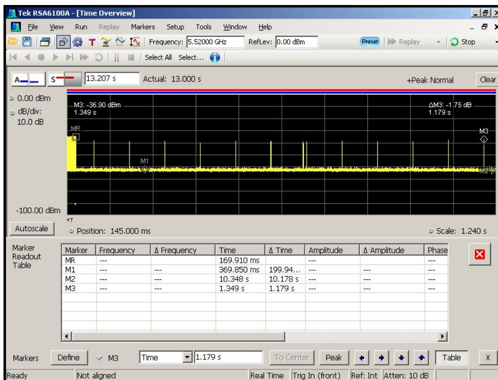
Figure 6-5. Channel Closing Transmission Time, Aggregate Time After 200ms
