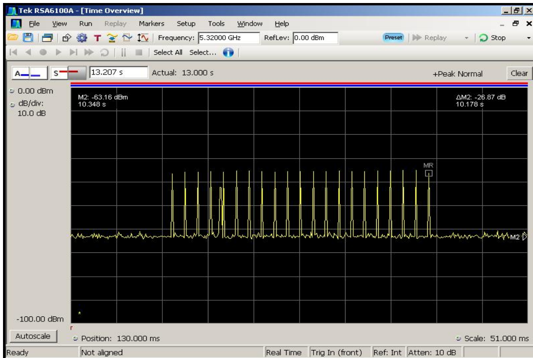
Figure 5-1. Type 1 Radar Pulse
