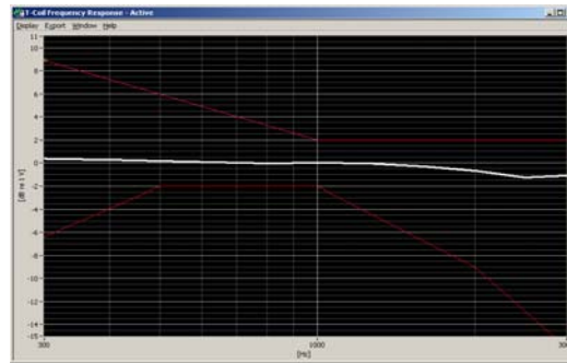
Figure 7-1 Axial Frequency Response
