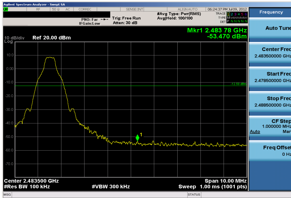
Plot 6-11. Band Edge Plot (Bluetooth with Hopping Disabled, 3Mbps – Ch. 78)
