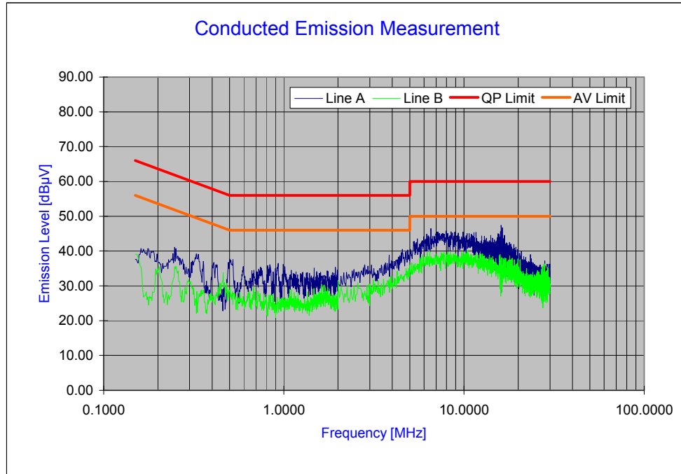
Plot 8-3. Line-Conducted Test Plot (Antenna Terminated)
