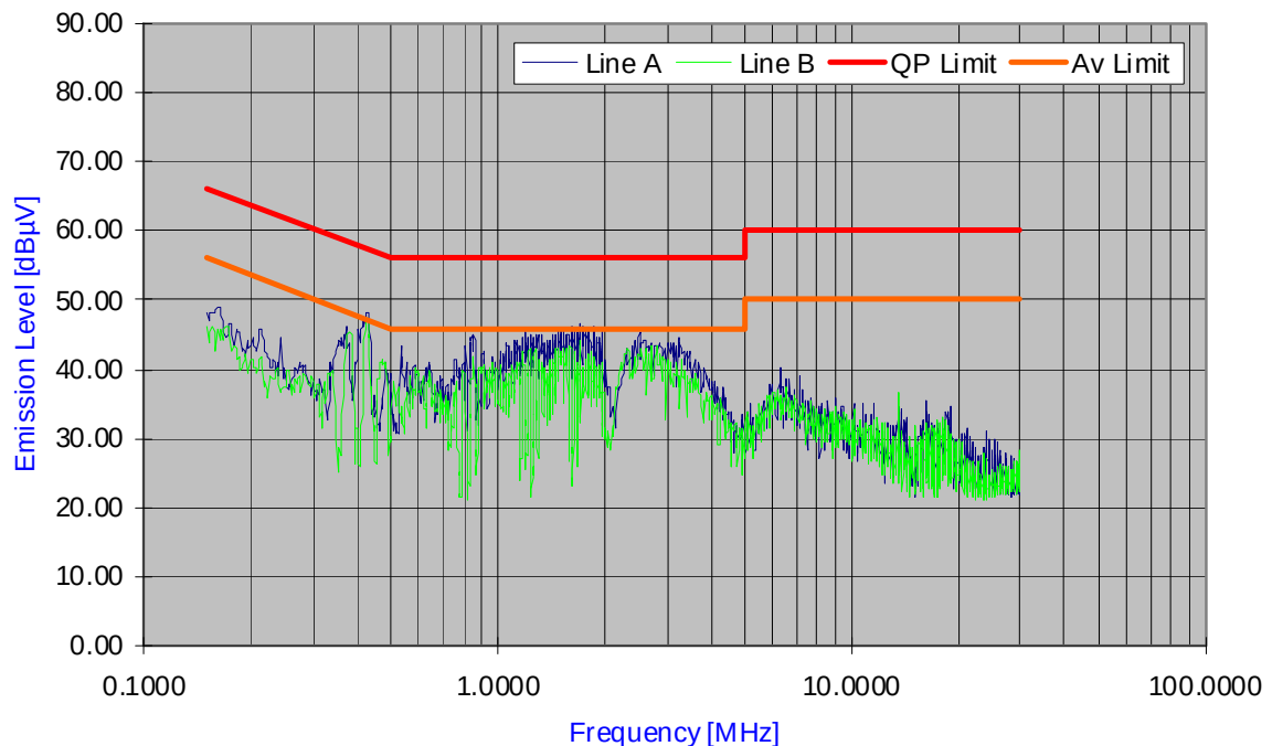
Plot 6-60. Line Conducted Plot with 802.11a
