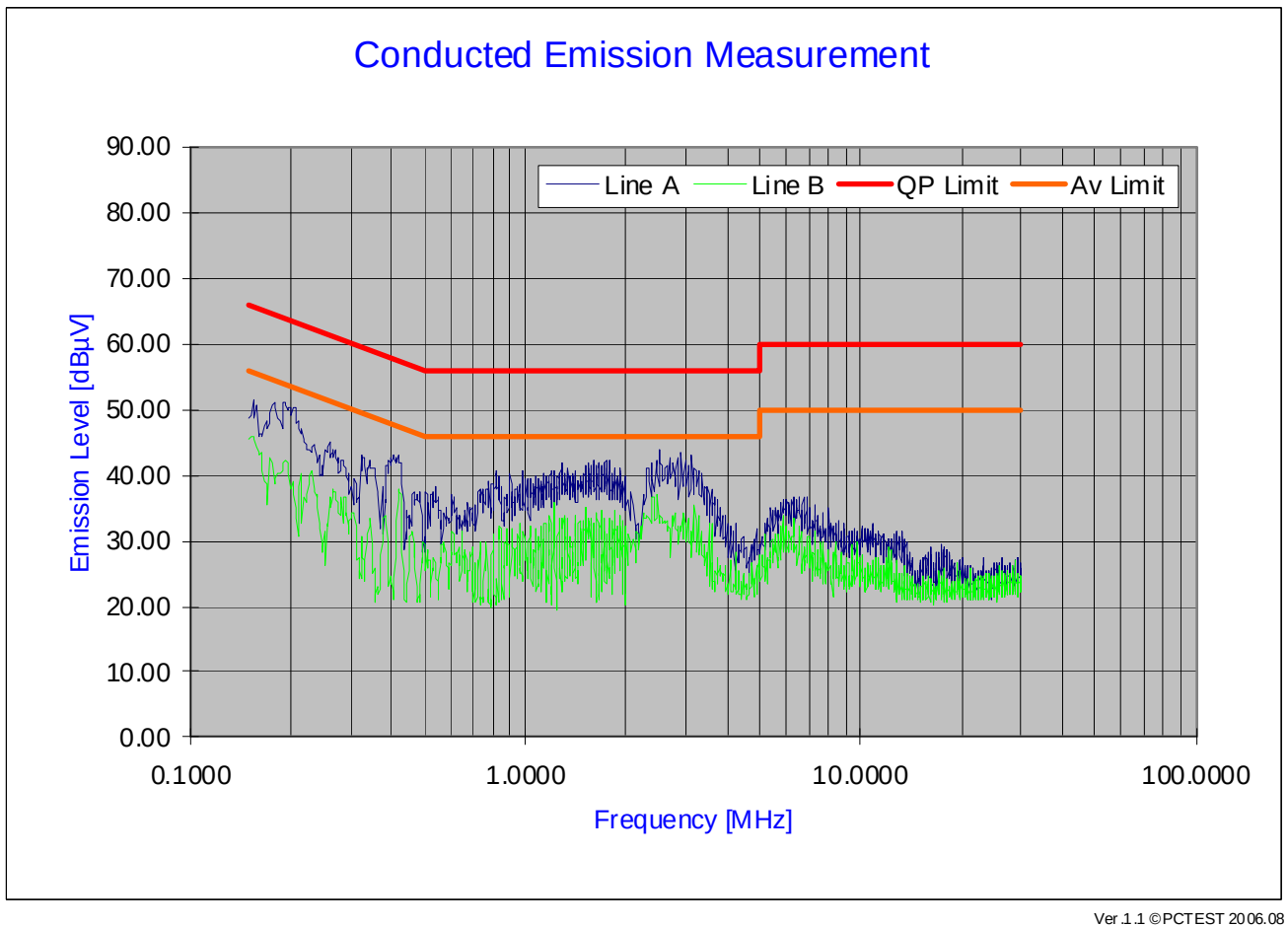
Plot 6-15. Line Conducted Plot with Bluetooth (LE)
