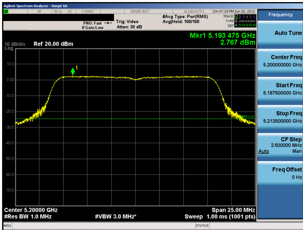
Plot 6-27. Peak Power Spectral Density Plot (802.11a (UNII Band 1) – Ch. 40)
