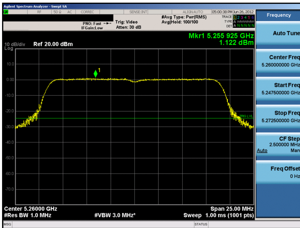
Plot 6-37. Peak Power Spectral Density Plot (20MHz BW 802.11n (UNII Band 2) – Ch. 52)
