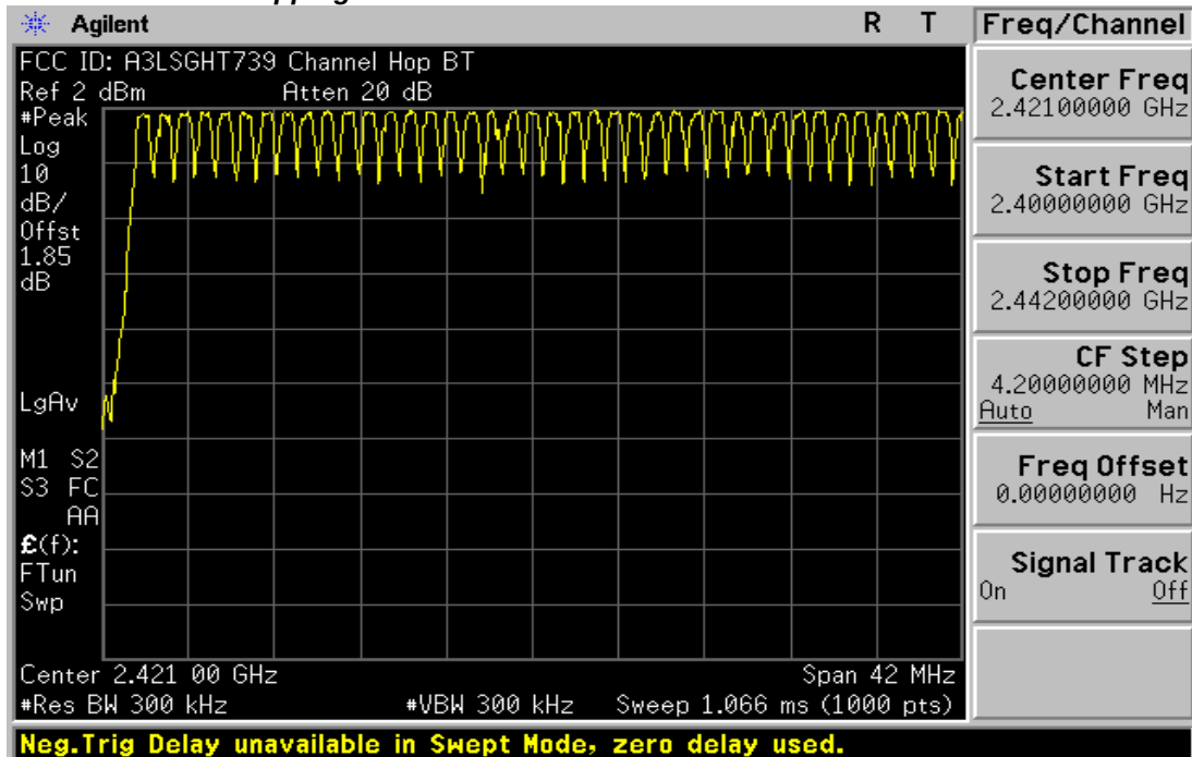
Plot 6-10. Low End Spectrum Channel Hopping Plot (Bluetooth)
