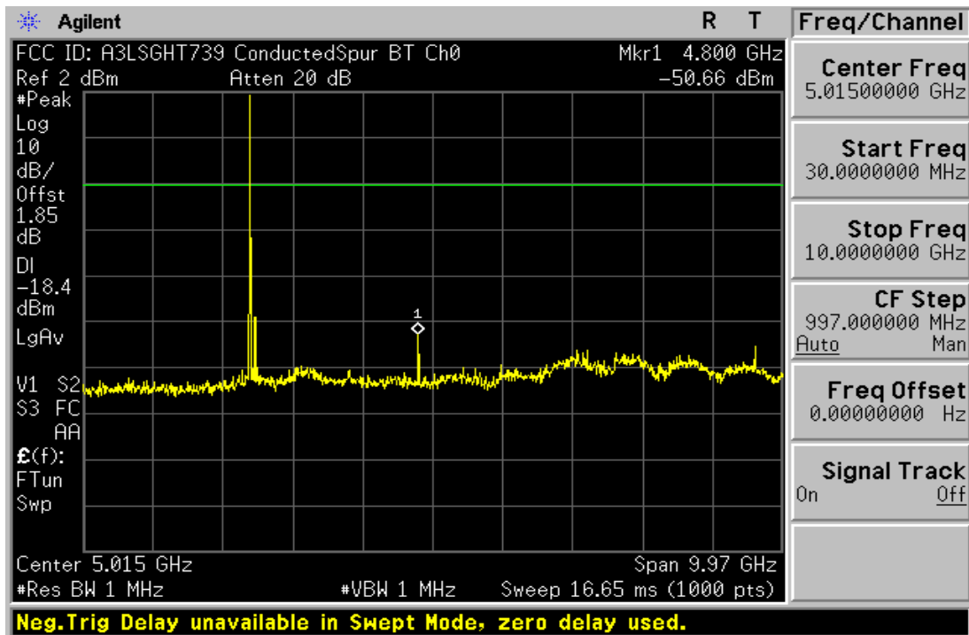
Plot 6-12. Conducted Spurious Plot (Bluetooth – Ch. 0)
