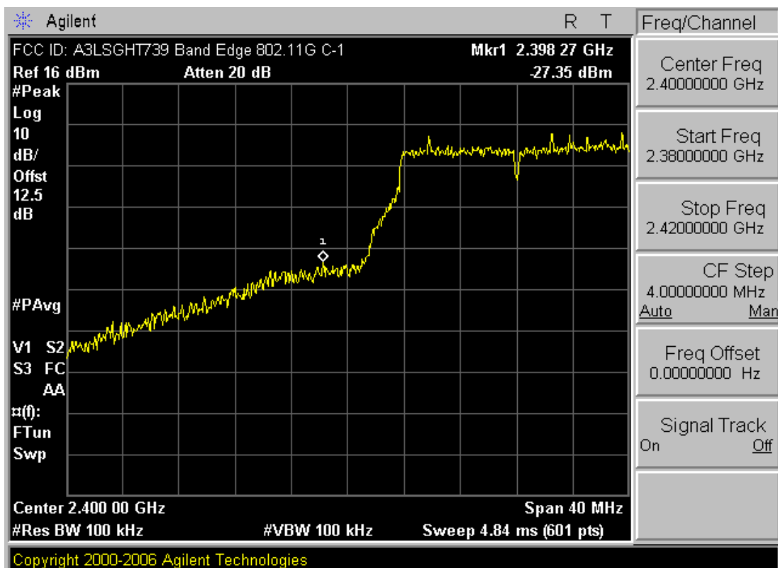
Plot 6-15. Band Edge Plot (802.11g – Ch. 1)
