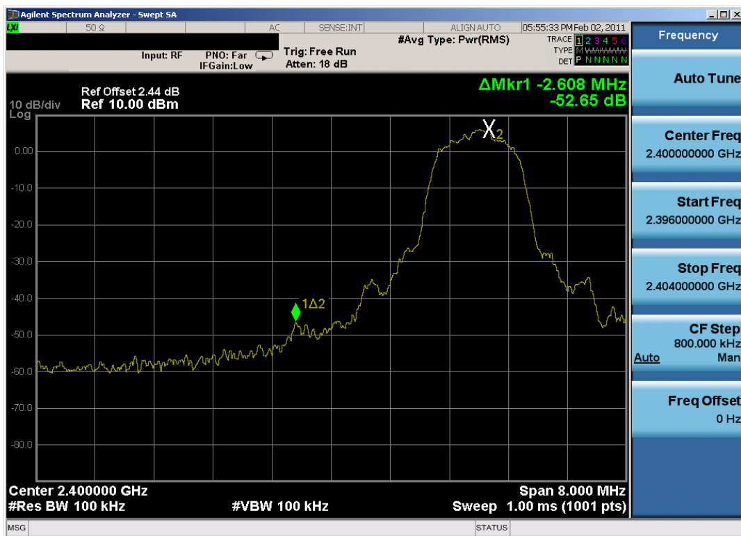
Plot 6-12. Band Edge Plot (Bluetooth, 2Mbps – Ch. 0)
