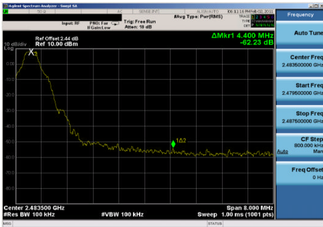
Plot 6-11. Band Edge Plot (Bluetooth, 1Mbps – Ch. 78)
