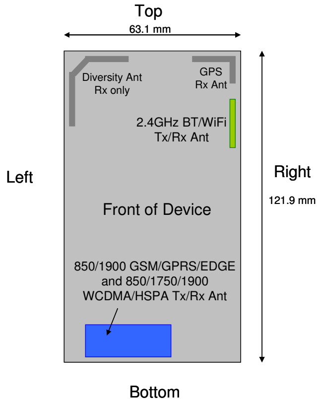
Figure 12-1 Identification of Sides for SAR Testing
