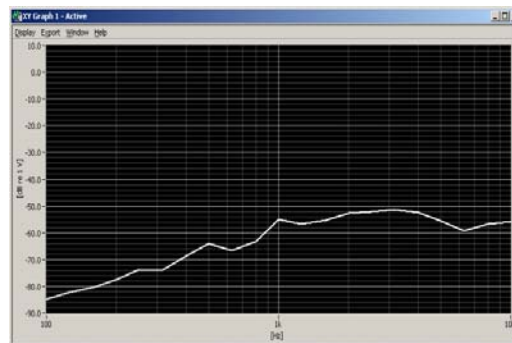
Figure 7-2 Worst-case ABM2 Plot for WD
