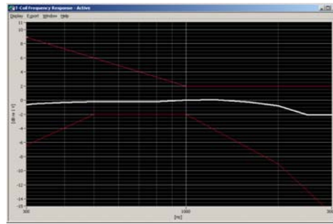
Figure 7-1 Axial Frequency Response
