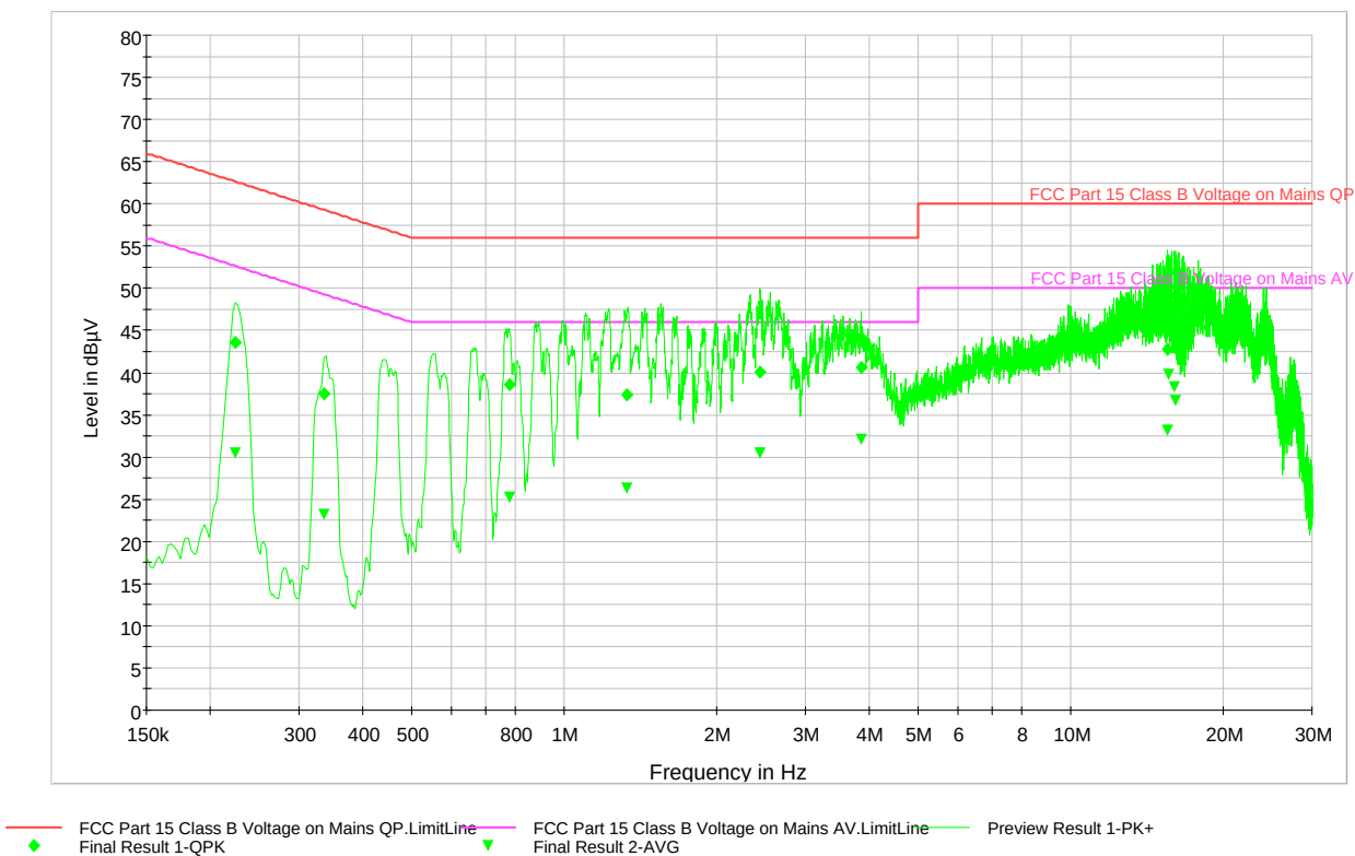
Plot 6-32. Line Conducted Plot with 802.11b (L2)
