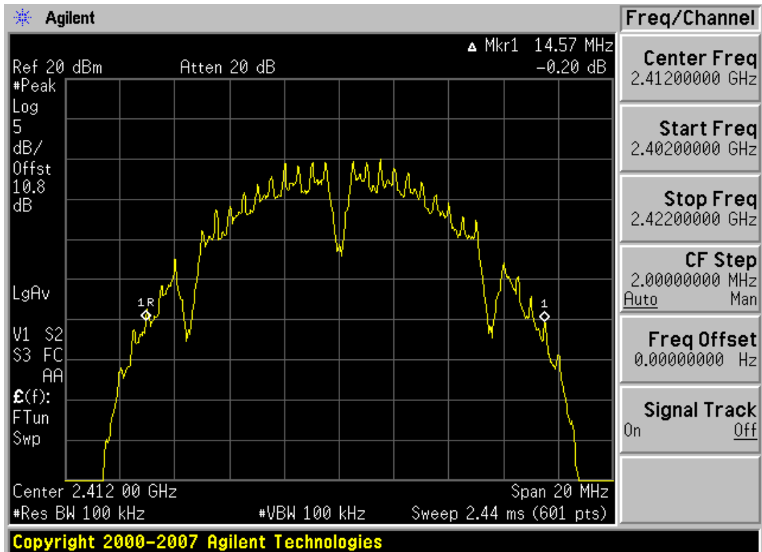
Plot 6-1. 6dB Bandwidth Plot (802.11b – Ch. 1)
