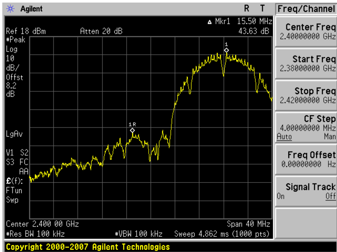
Plot 6-31. Band Edge Plot (802.11b – Ch. 1)
