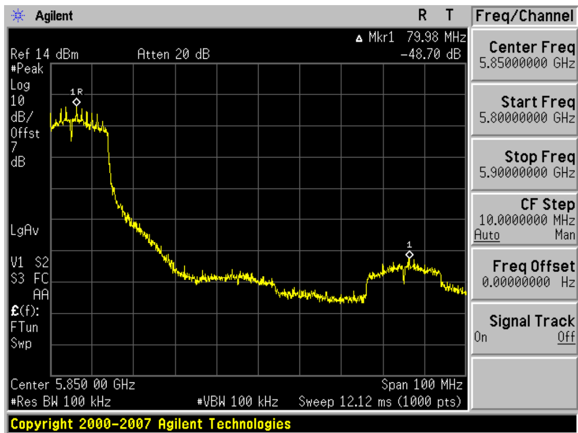
Plot 6-40. Band Edge Plot (802.11n (5.8GHz) – Ch. 161)
