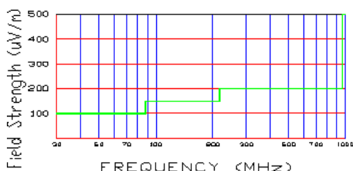
Figure 6-6. 3-Meter Limits
