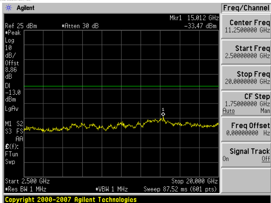
Plot 7-55. Conducted Spurious Plot (AWS WCDMA Mode – Ch. 1862)
