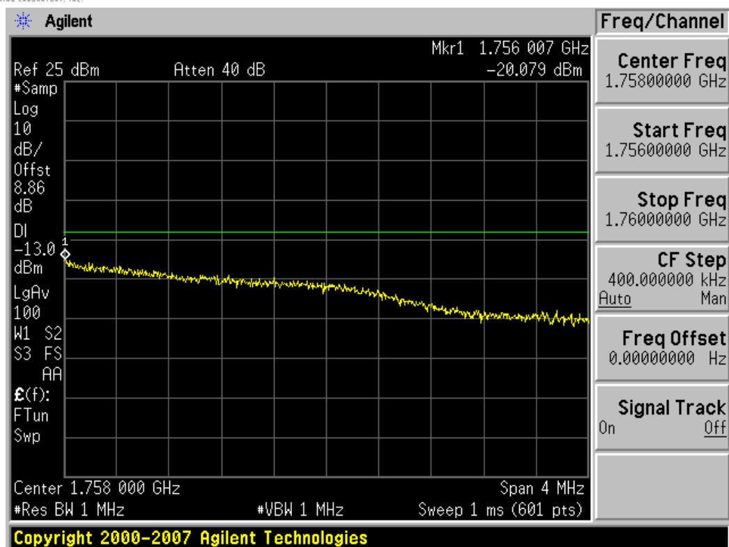
Plot 7-57. 4MHz Span Plot (AWS WCDMA Mode – Ch. 1862)
