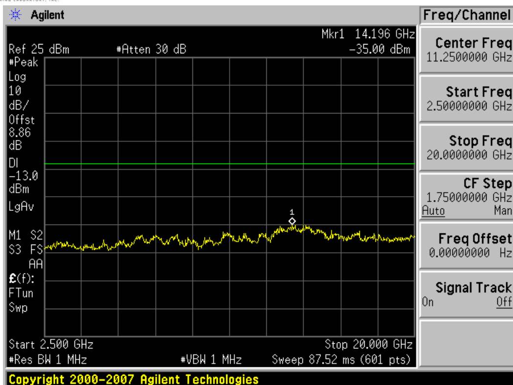
Plot 7-47. Conducted Spurious Plot (AWS WCDMA Mode – Ch. 1312)
