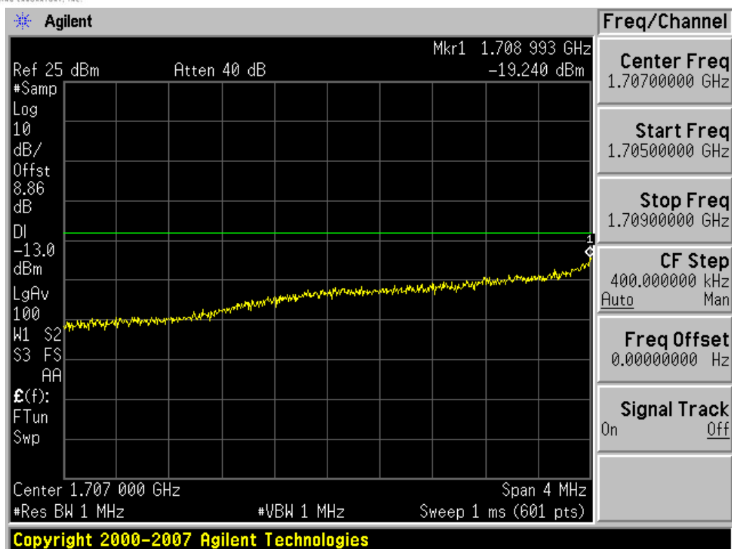
Plot 7-49. 4MHz Span Plot (AWS WCDMA Mode – Ch. 1312)
