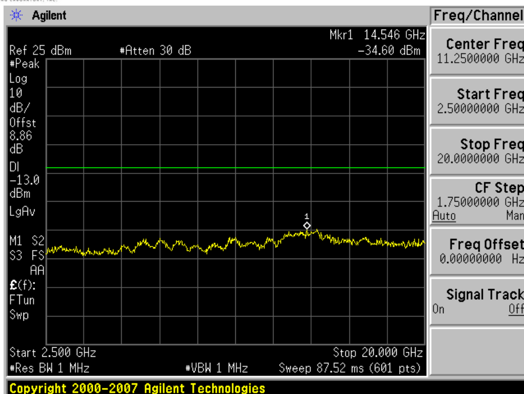
Plot 7-51. Conducted Spurious Plot (AWS WCDMA Mode – Ch. 1412)
