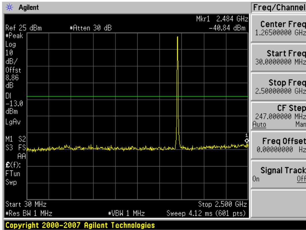
Plot 7-46. Conducted Spurious Plot (AWS WCDMA Mode – Ch. 1312)
