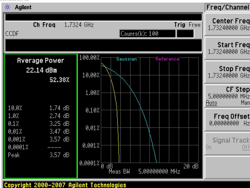
Plot 7-53. Peak-Average Ratio Plot (AWS WCDMA Mode – Ch. 1412)
