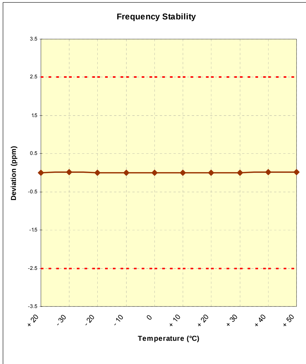
Figure 6-5. Frequency Stability Graph (AWS WCDMA Mode – Ch. 1412)
