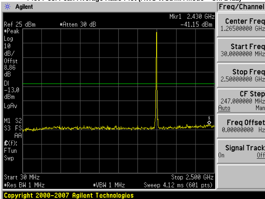
Plot 7-54. Conducted Spurious Plot (AWS WCDMA Mode – Ch. 1862)
