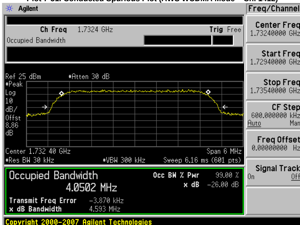
Plot 7-52. Occupied Bandwidth Plot (AWS WCDMA Mode – Ch. 1412)
