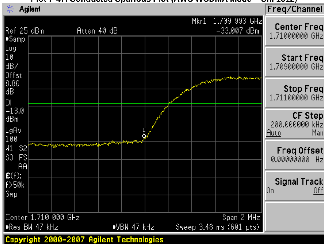
Plot 7-48. Band Edge Plot (AWS WCDMA Mode – Ch. 1312)
