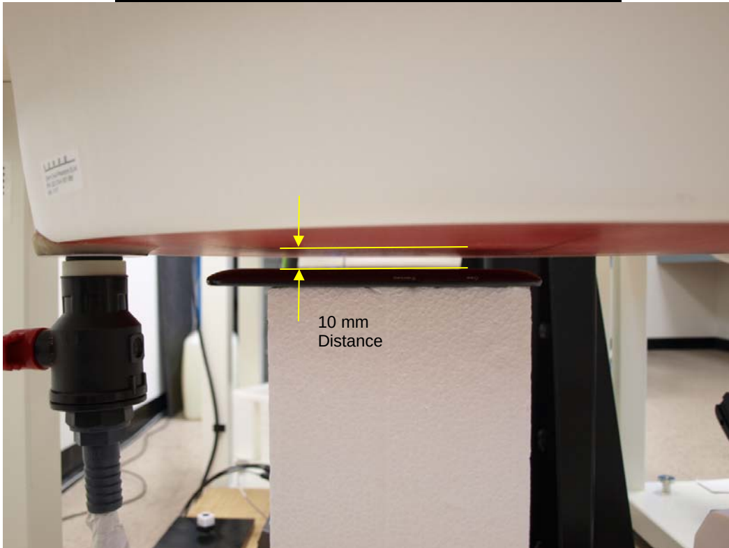
Rear/Base with 10 mm separation distance (Full Power)
