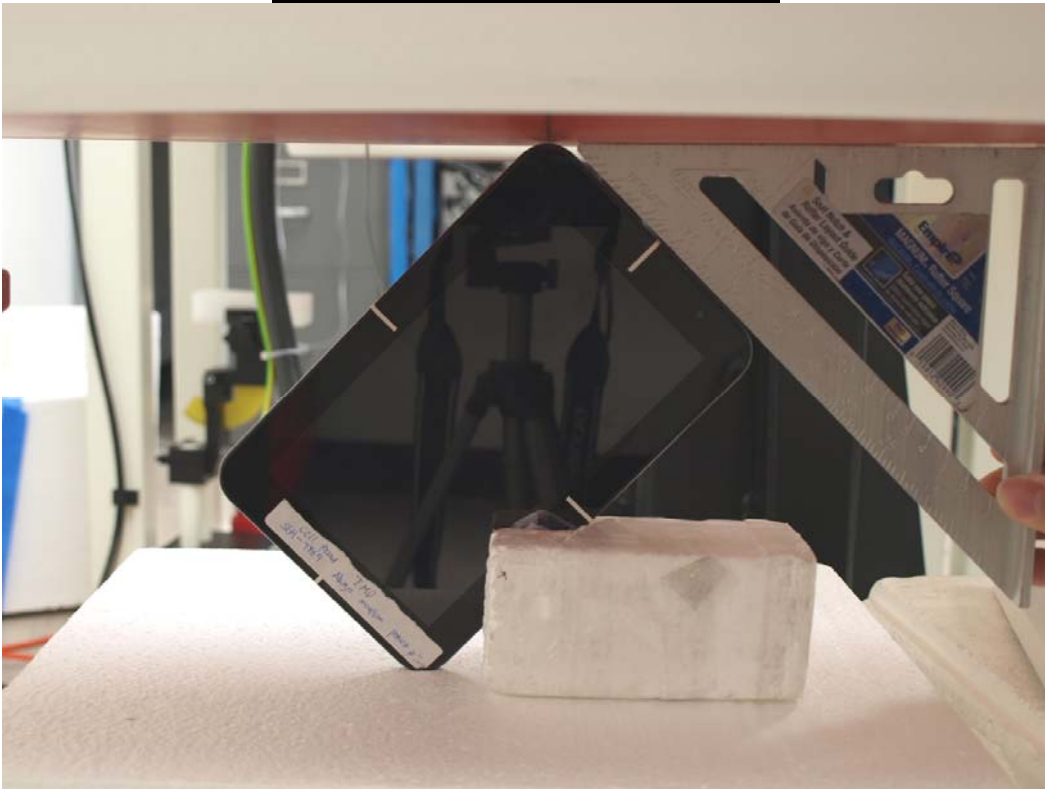
Top/Sec. Landscape (45°) (Full Power)
