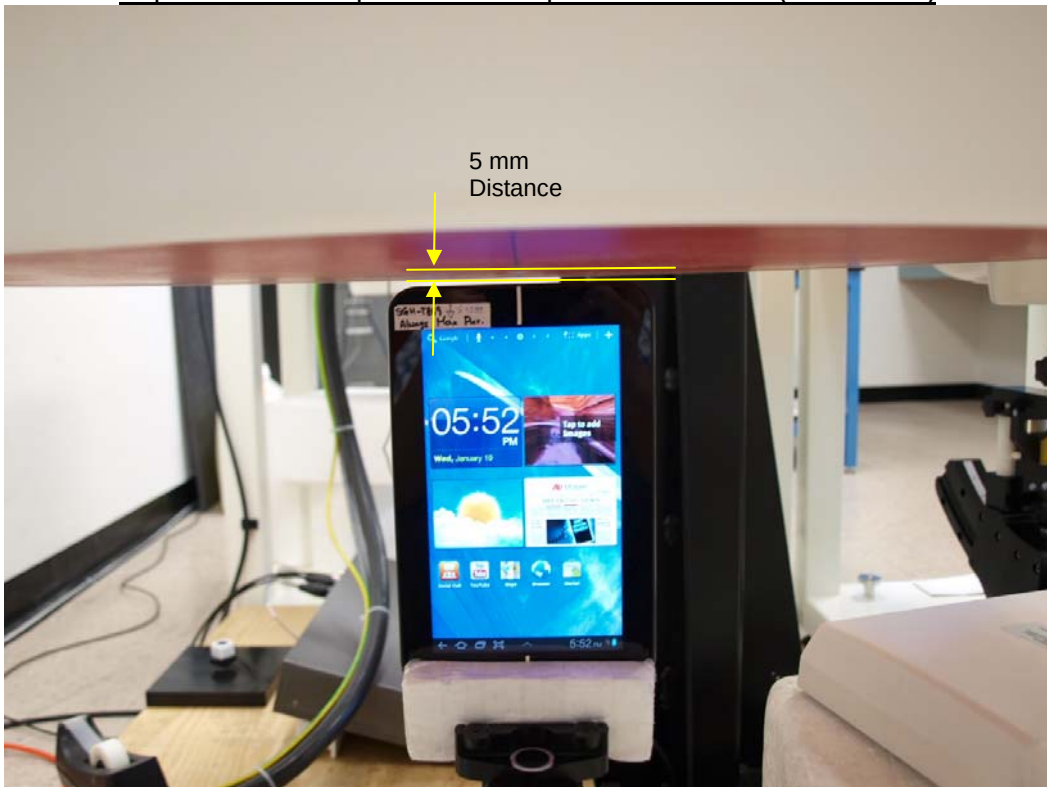
Top/Sec. Landscape w/ 5 mm separation distance (Full Power)
