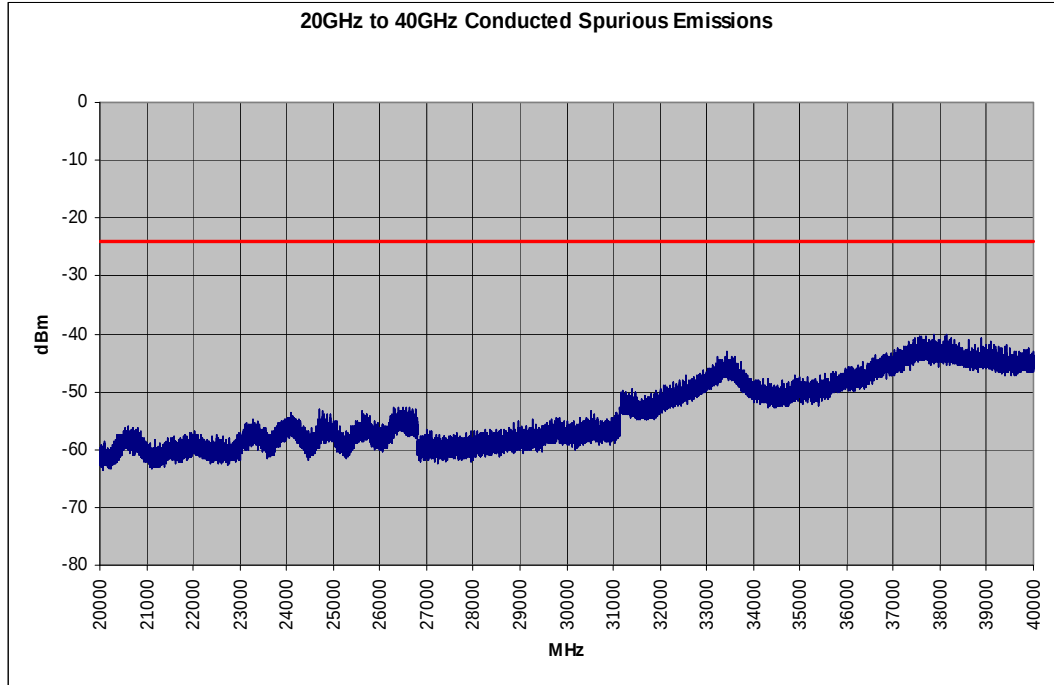
Plot 6-48. Conducted Spurious Plot (802.11a – Ch. 149)
