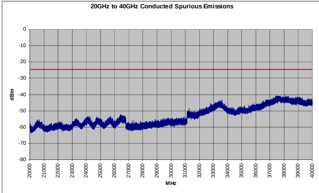
Plot 6-52. Conducted Spurious Plot (802.11a – Ch. 165)
