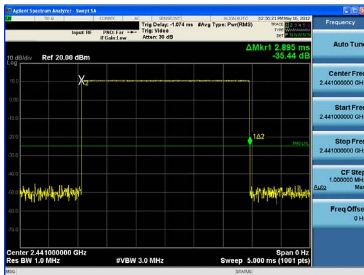
Plot 6-15. Time of Occupancy Plot (Bluetooth)
