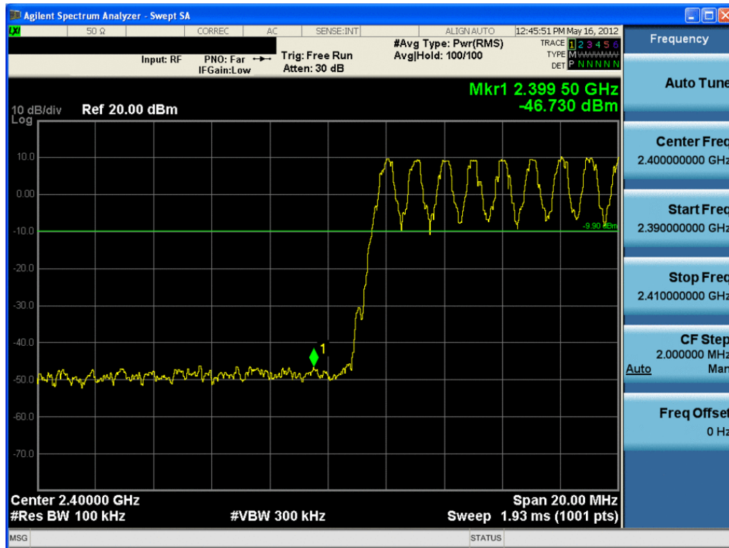
Plot 6-12. Band Edge Plot (Bluetooth with Hopping Enabled, 3Mbps – Ch. 0)
