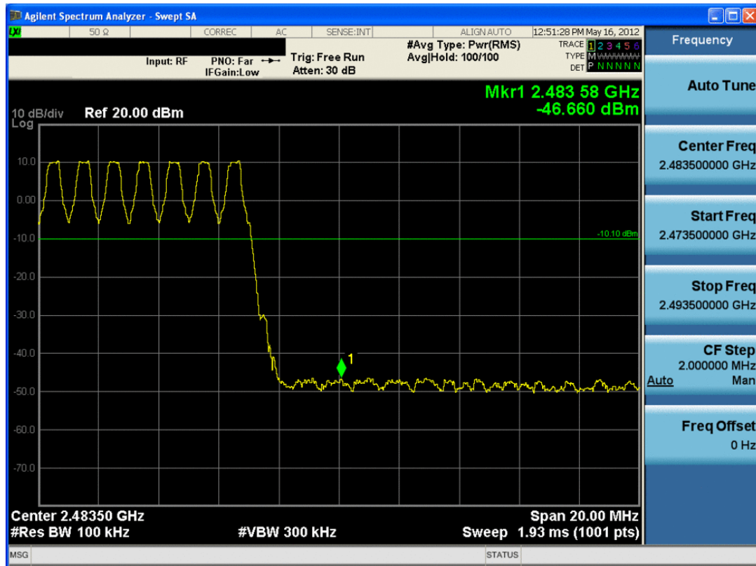
Plot 6-13. Band Edge Plot (Bluetooth with Hopping Enabled, 3Mbps – Ch. 78)
