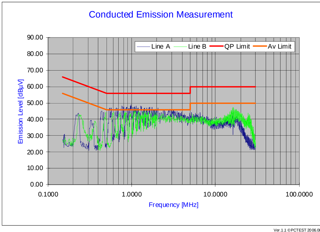
Plot 6-24. Line Conducted Plot with Bluetooth
