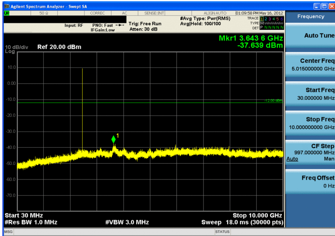
Plot 6-18. Conducted Spurious Plot (Bluetooth, 3Mbps – Ch. 0)
