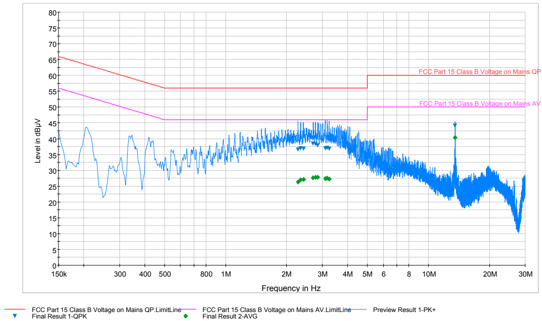
Plot 8-7. Line-Conducted Test Plot with NFC – Line 1
