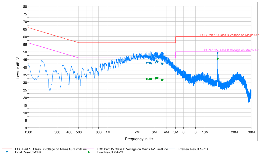
Plot 8-8. Line-Conducted Test Plot with NFC – Line N
