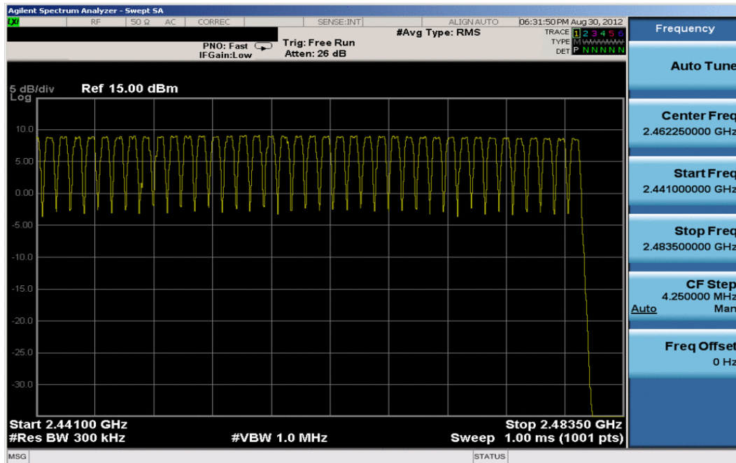
Plot 6-26. High End Spectrum Channel Hopping Plot (Bluetooth)
