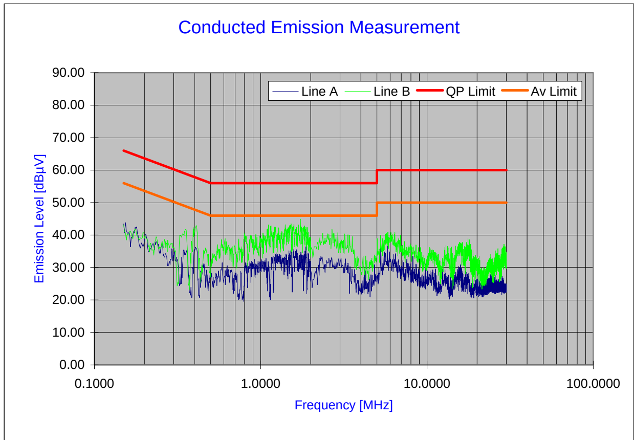
Plot 6-59. Line Conducted Plot with 802.11b
