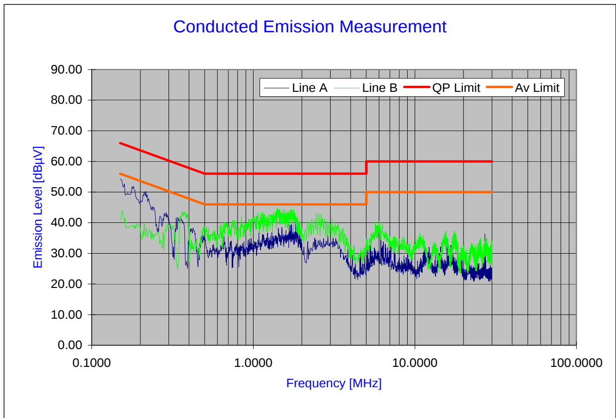
Plot 6-33. Line Conducted Plot with Bluetooth
