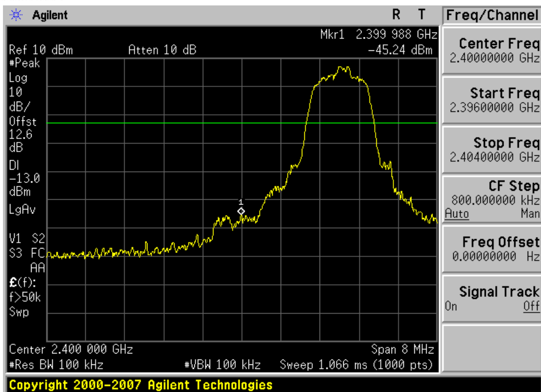
Plot 6-6. Band Edge Plot (Bluetooth 3.0 with Enhanced Data Rates – Ch. 0)
