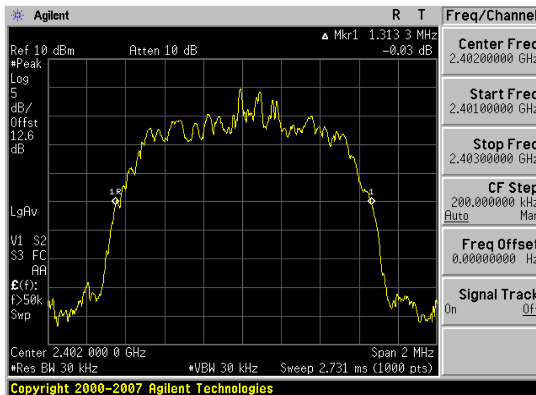
Plot 6-1. 20dB Bandwidth Plot (Bluetooth 3.0 with Enhanced Data Rates – Ch. 0)
