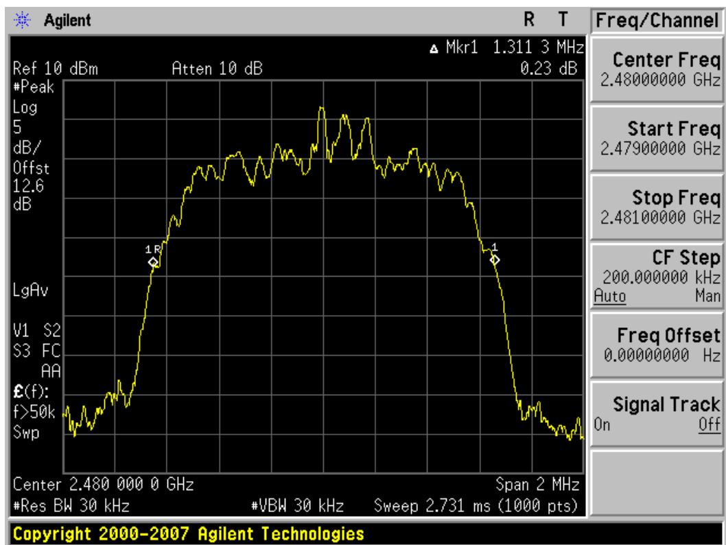
Plot 6-3. 20dB Bandwidth Plot (Bluetooth 3.0 with Enhanced Data Rates – Ch. 78)
