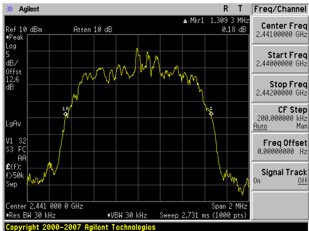
Plot 6-2. 20dB Bandwidth Plot (Bluetooth 3.0 with Enhanced Data Rates – Ch. 39)
