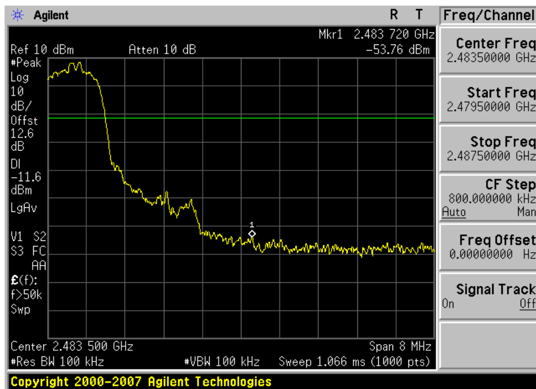
Plot 6-7. Band Edge Plot (Bluetooth 3.0 with Enhanced Data Rates – Ch. 78)
