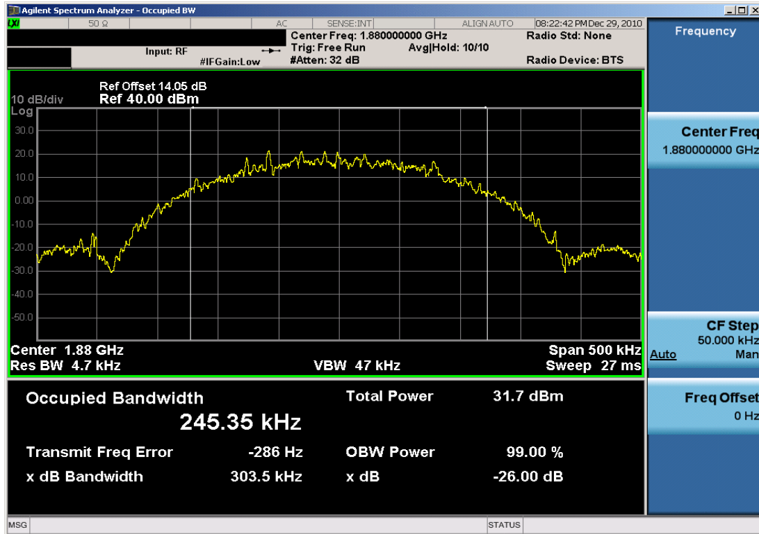
Plot 7-21. Occupied Bandwidth Plot (EDGE1900 Mode – Ch. 661)
