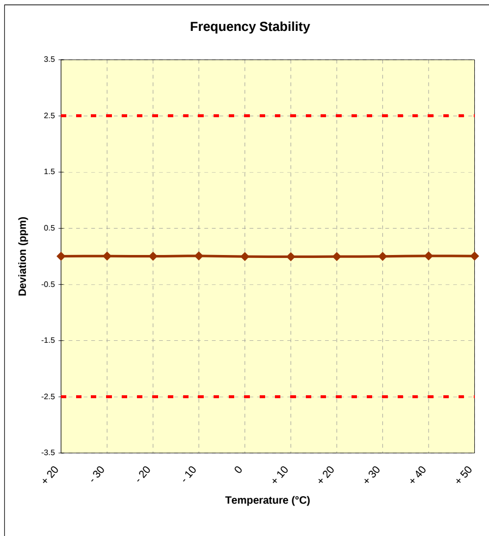
Figure 6-4. Frequency Stability Graph (AWS WCDMA Mode – Ch. 1412)
