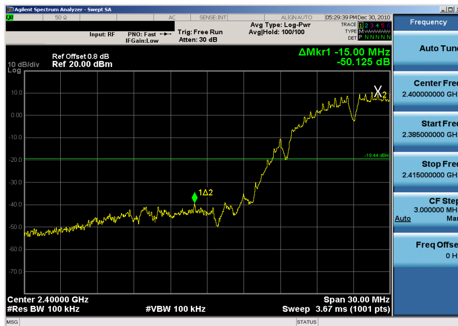
Plot 6-19. Band Edge Plot (802.11b – Ch. 1)
