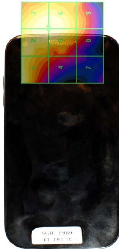
Figure 17-5 H-Field WD Scan overlay
