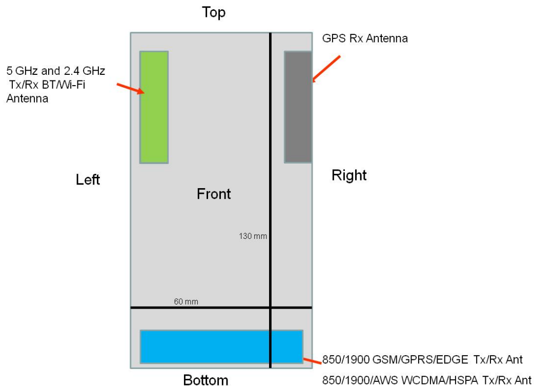
Figure 13-1 Identification of Sides for SAR Testing
