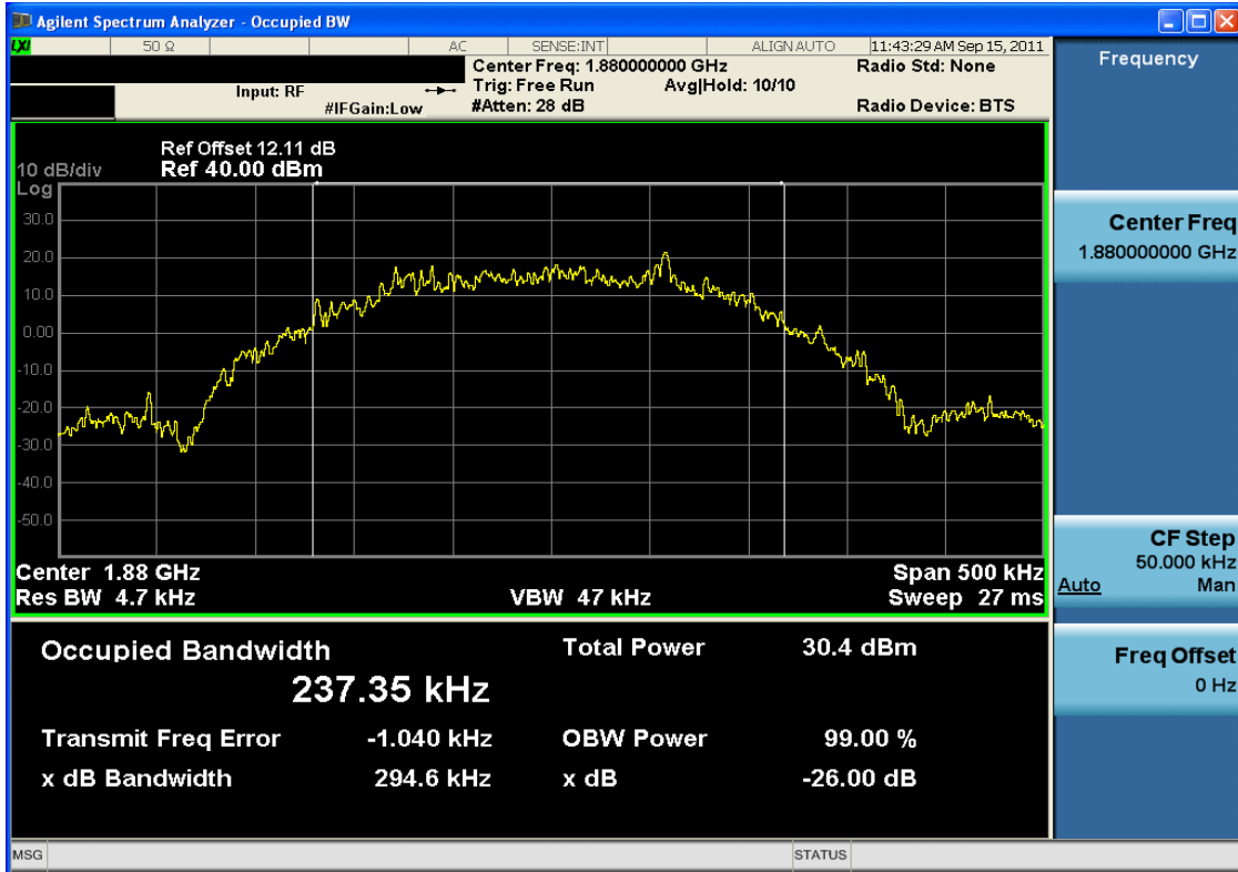
Plot 7-21. Occupied Bandwidth Plot, Average Detector (EDGE1900 Mode – Ch. 661)
