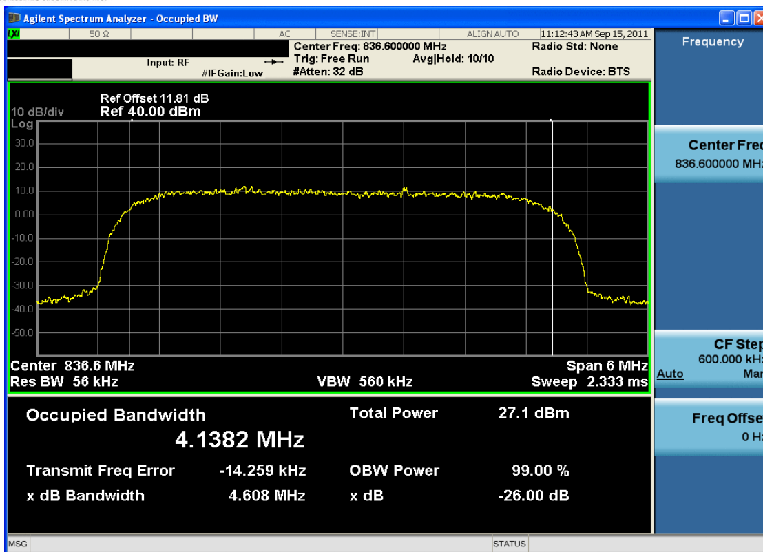
Plot 7-29. Occupied Bandwidth Plot, Average Detector (Cellular WCDMA Mode – Ch. 4183)
