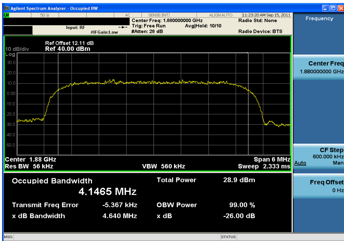
Plot 7-40. Occupied Bandwidth Plot, Average Detector (PCS WCDMA Mode – Ch. 9400)
