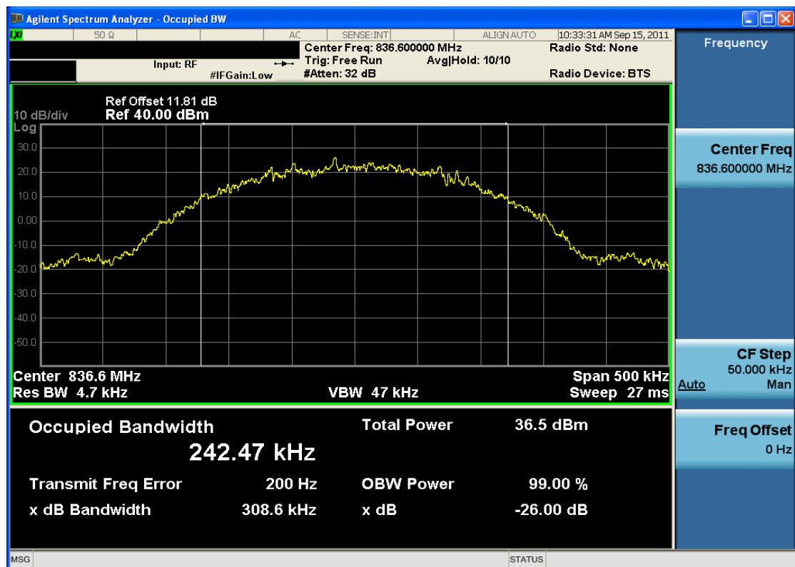
Plot 7-6. Occupied Bandwidth Plot, Average Detector (Cellular GSM Mode – Ch. 190)
