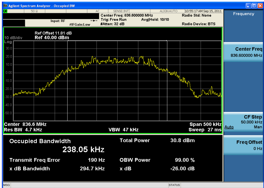
Plot 7-10. Occupied Bandwidth Plot, Average Detector (EDGE850 Mode – Ch. 190)
