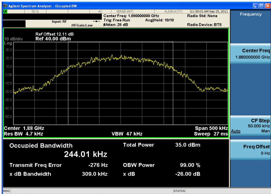
Plot 7-16. Occupied Bandwidth Plot, Average Detector (PCS GSM Mode – Ch. 661)
