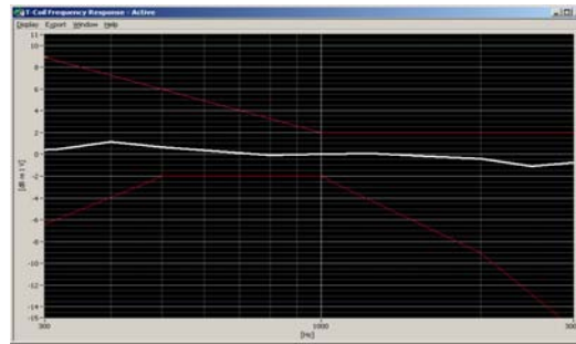
Figure 7-1 Axial Frequency Response
