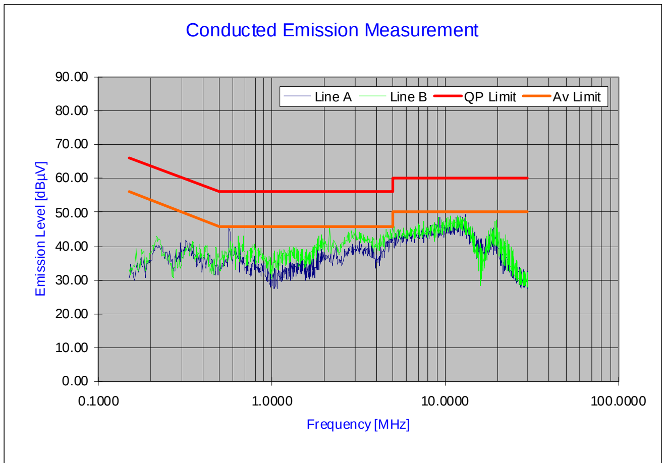
Plot 6-56. Line Conducted Plot with 802.11b
