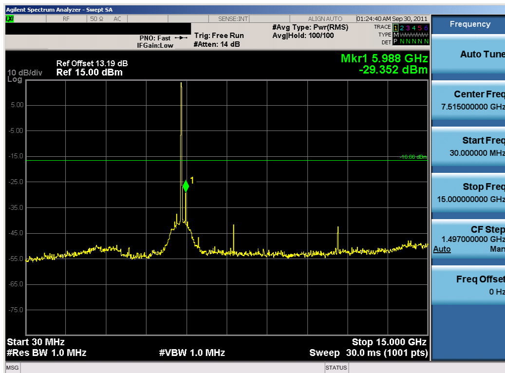
Plot 6-53. Conducted Spurious Plot (802.11a – Ch. 165)
