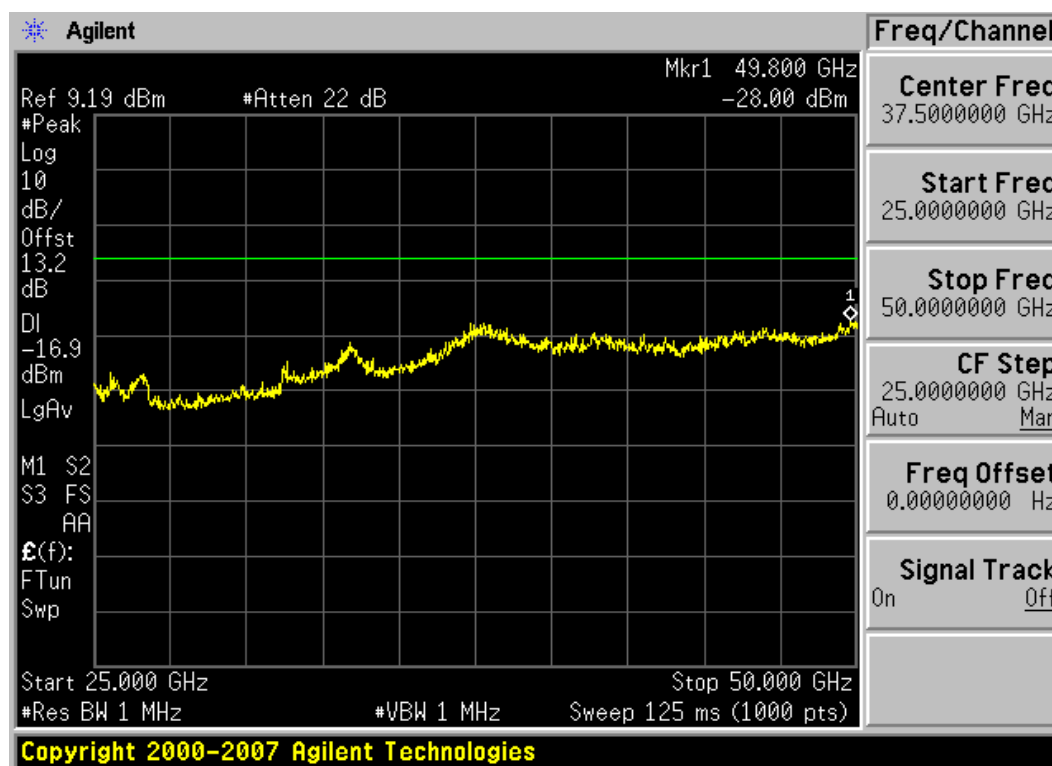
Plot 6-49. Conducted Spurious Plot (802.11a – Ch. 149)
