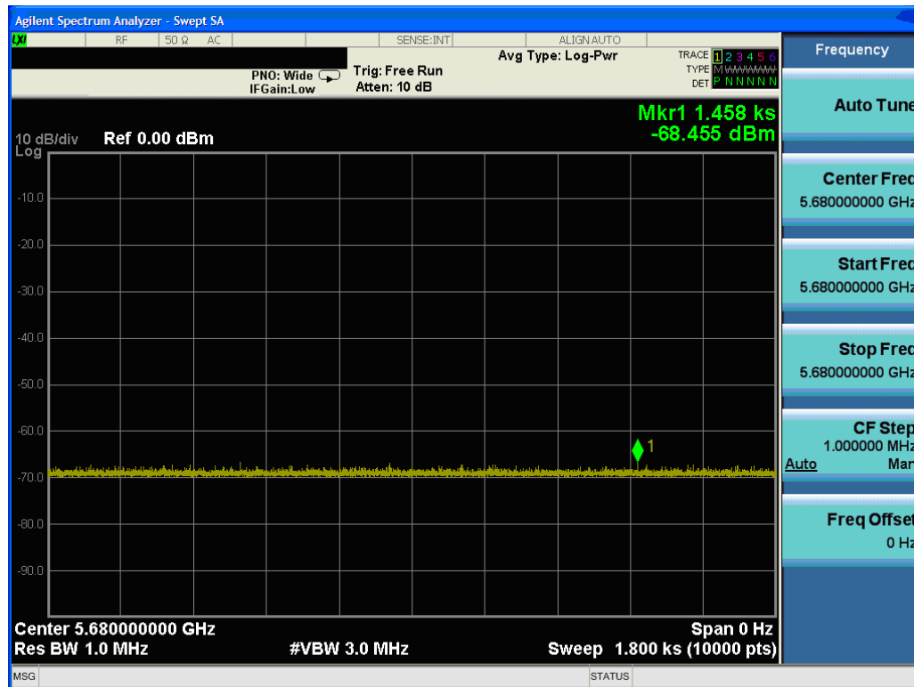
Figure 6-7 Non-occupancy Period After Startup - 30min
