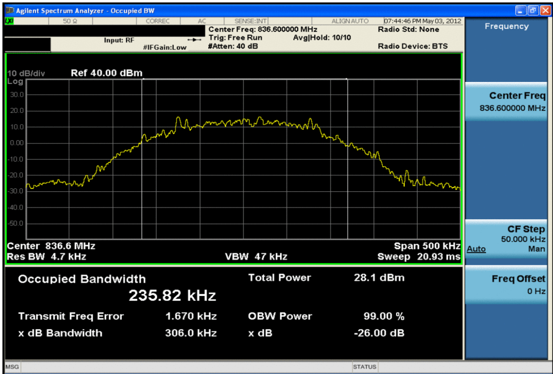
Plot 7-10. Occupied Bandwidth Plot (EDGE850 Mode – Ch. 190)
