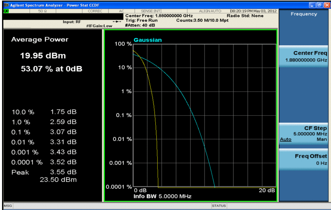
Plot 7-41. Peak-Average Ratio Plot (PCS WCDMA Mode – Ch. 9400)
