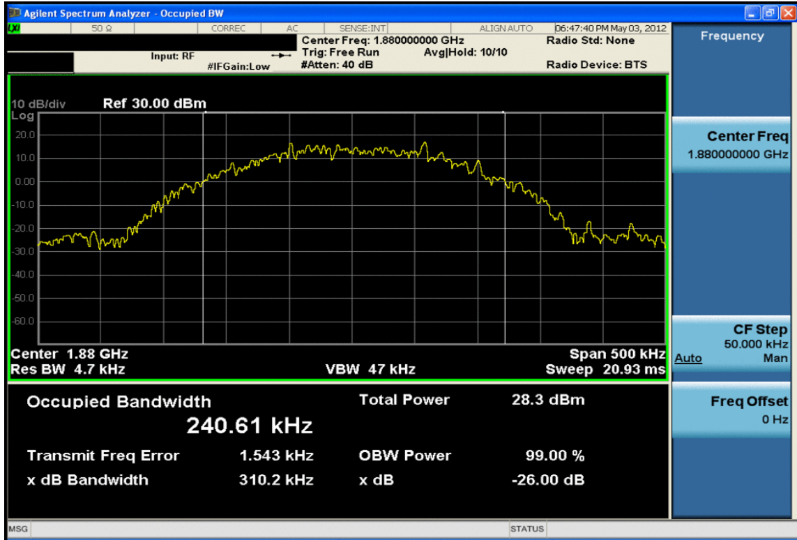
Plot 7-21. Occupied Bandwidth Plot (EDGE1900 Mode – Ch. 661)
