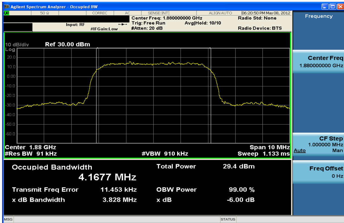
Plot 7-40. Occupied Bandwidth Plot (PCS WCDMA Mode – Ch. 9400)
