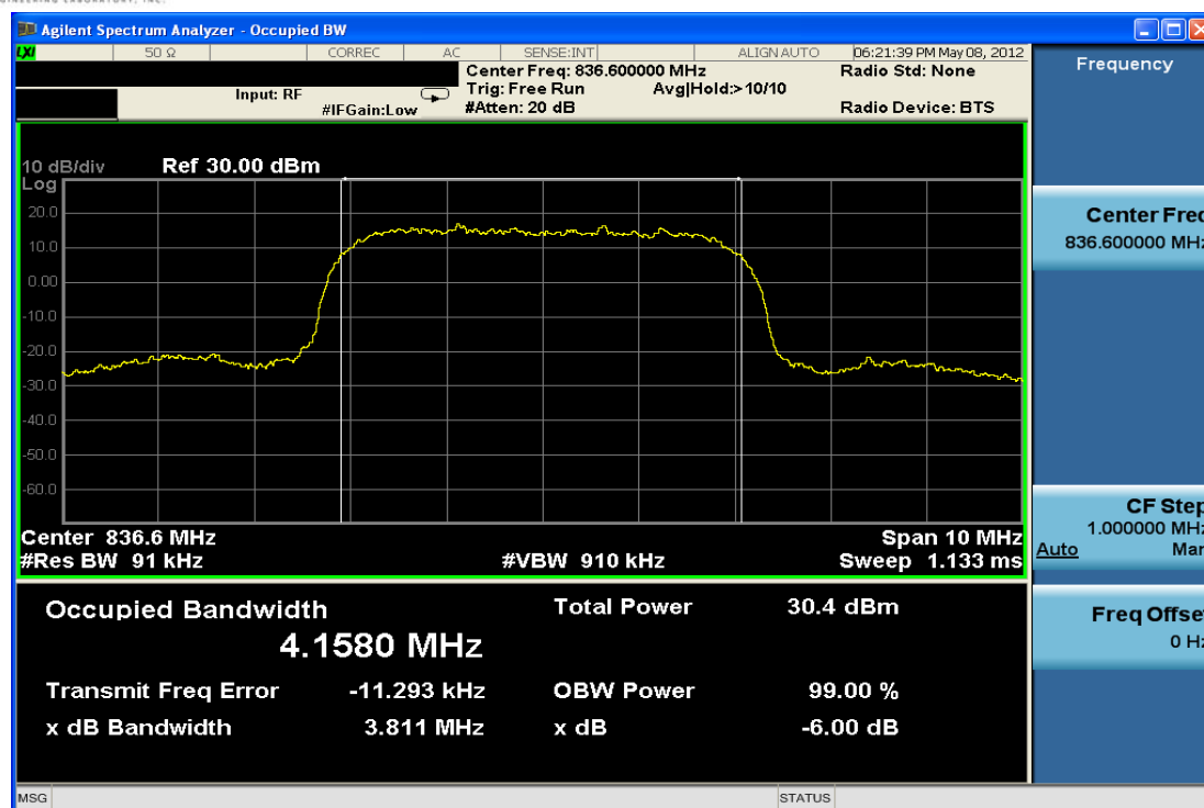
Plot 7-29. Occupied Bandwidth Plot (Cellular WCDMA Mode – Ch. 4183)
