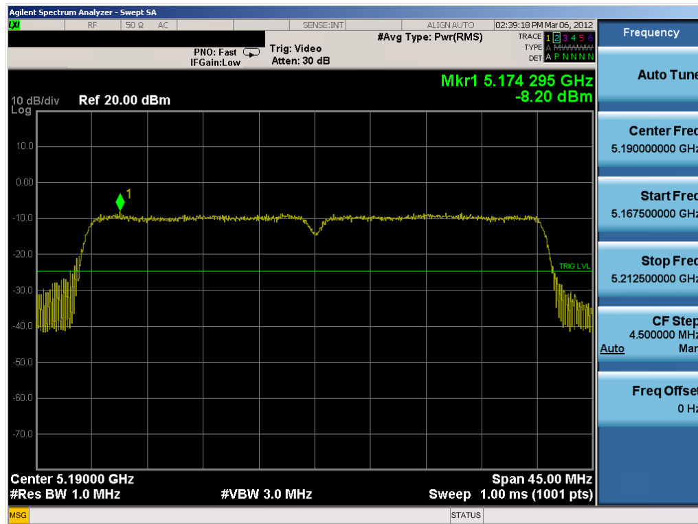
Plot 6-44. Peak Power Spectral Density Plot (802.11n (UNII Band 2 – 40MHz BW) – Ch. 38)
