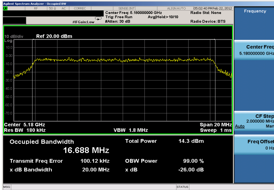
Plot 6-1. 26dB Bandwidth Plot (802.11a (UNII Band 1) – Ch. 36)
