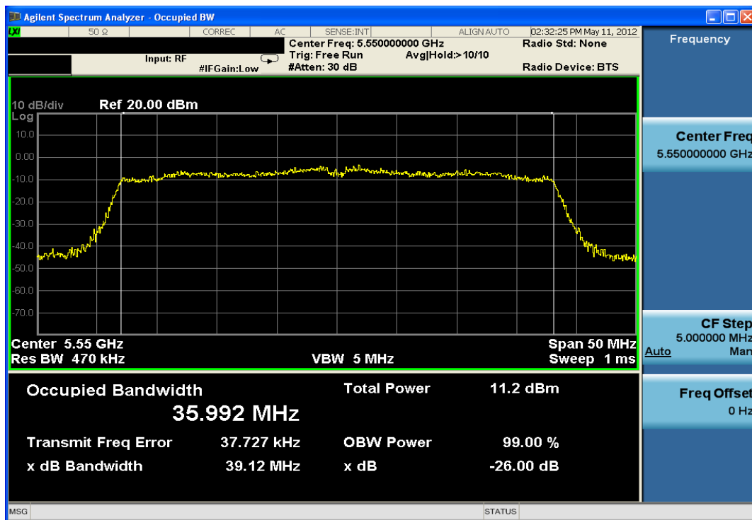
Plot 6-24. 26dB Bandwidth Plot (802.11n (UNII Band 3 – 40MHz BW) – Ch. 110)
