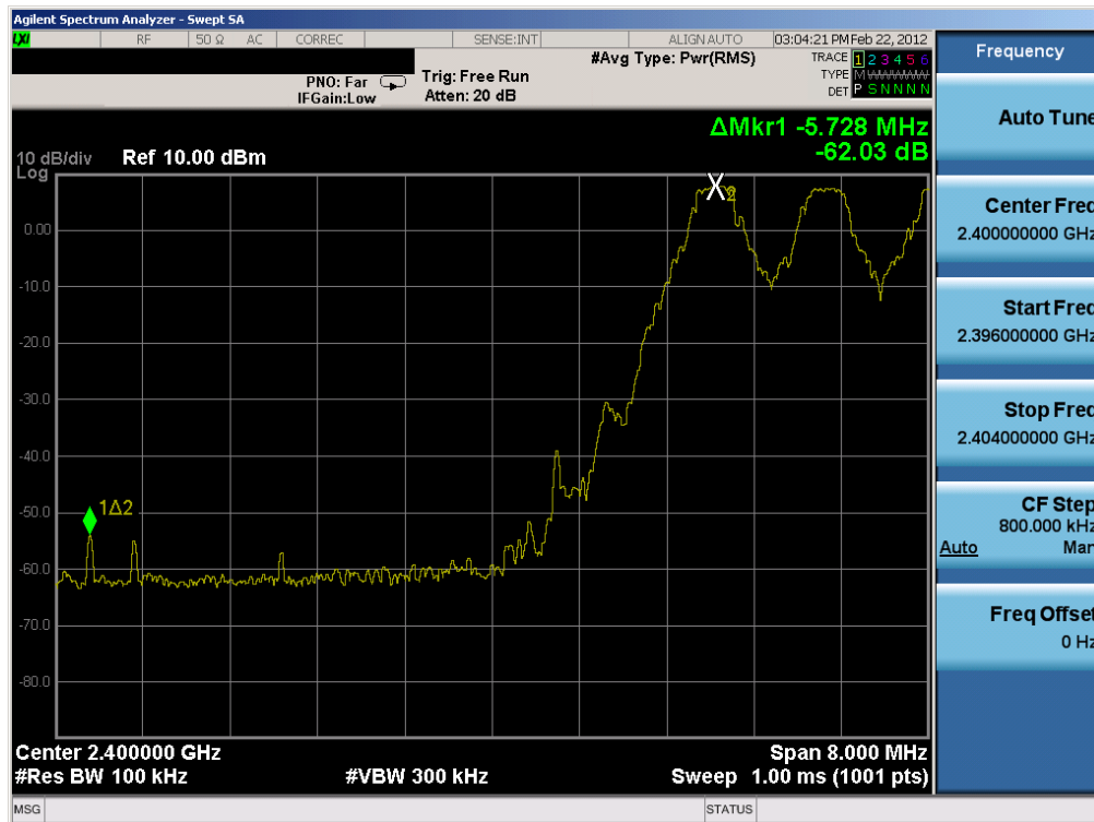
Plot 6-12. Band Edge Plot (Bluetooth with Hopping Enabled, 1Mbps – Ch. 0)
