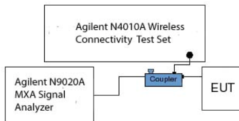
Figure 6-2. Test Instrument & Measurement Setup
