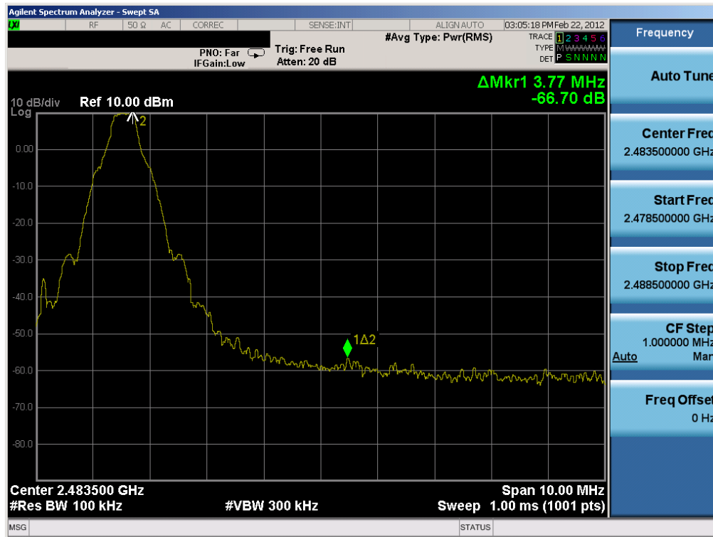
Plot 6-11. Band Edge Plot (Bluetooth with Hopping Disabled, 1Mbps – Ch. 78)
