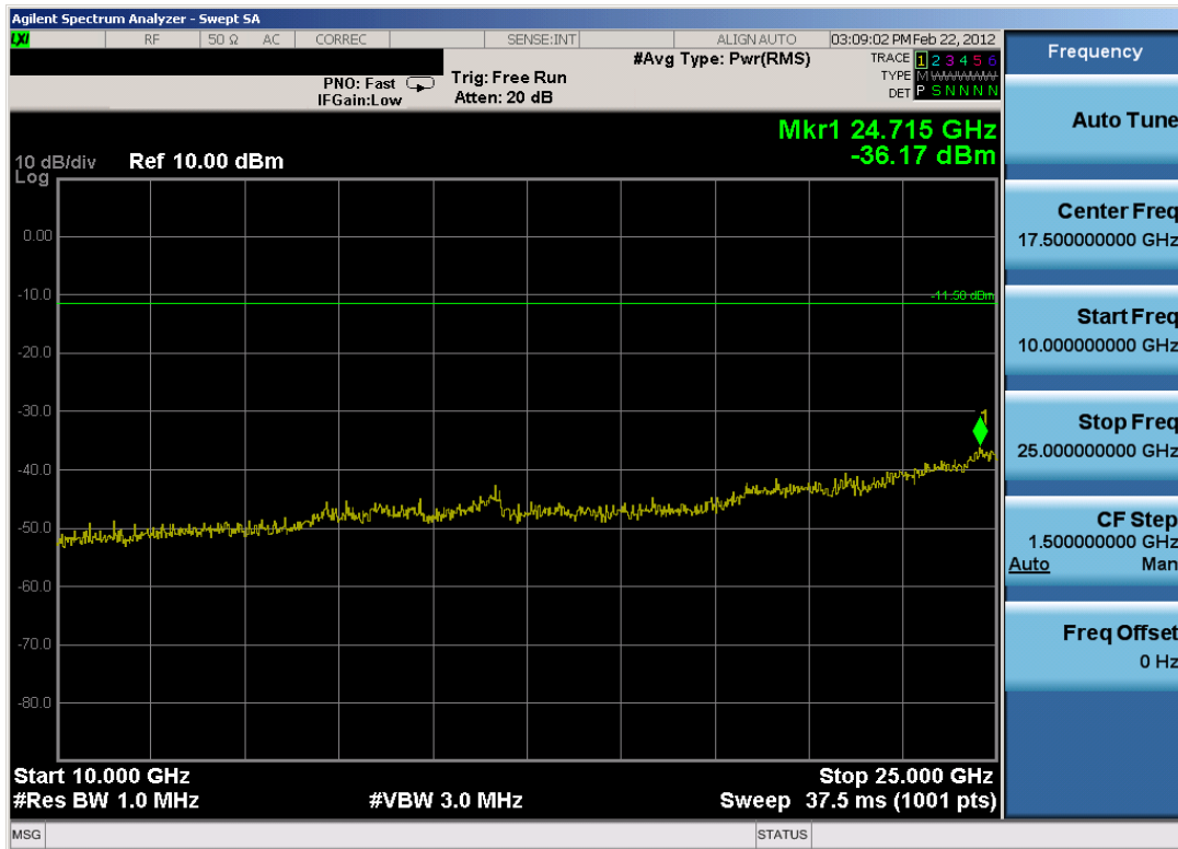
Plot 6-21. Conducted Spurious Plot (Bluetooth, 1Mbps – Ch. 39)
