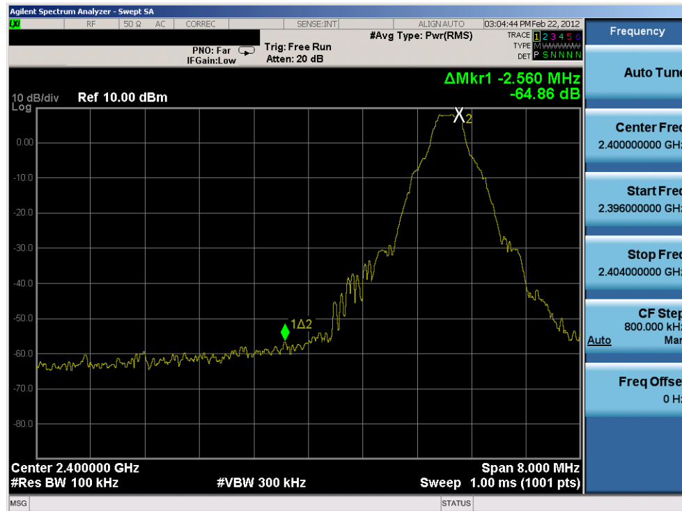
Plot 6-10. Band Edge Plot (Bluetooth with Hopping Disabled, 1Mbps – Ch. 0)
