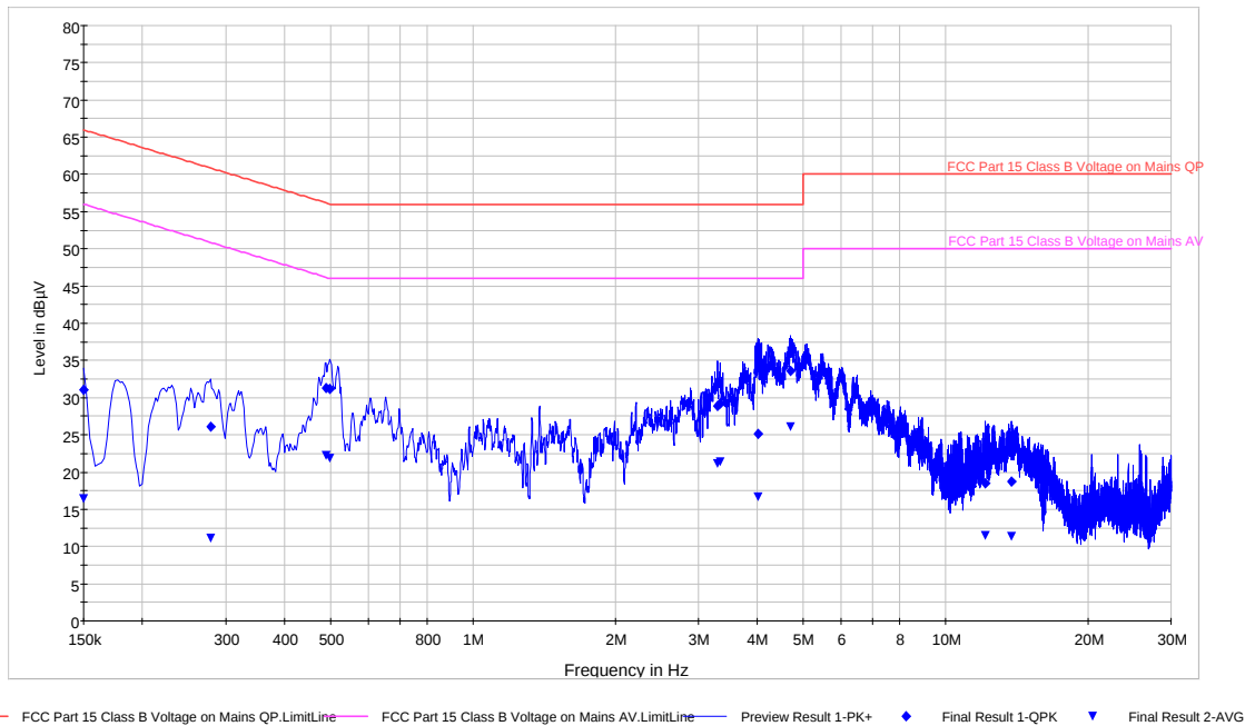
Plot 6-24. Line Conducted Plot with Bluetooth – Line 1
