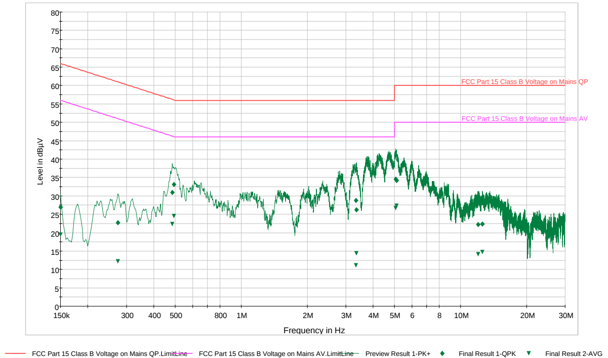
Plot 6-25. Line Conducted Plot with Bluetooth – Line N
