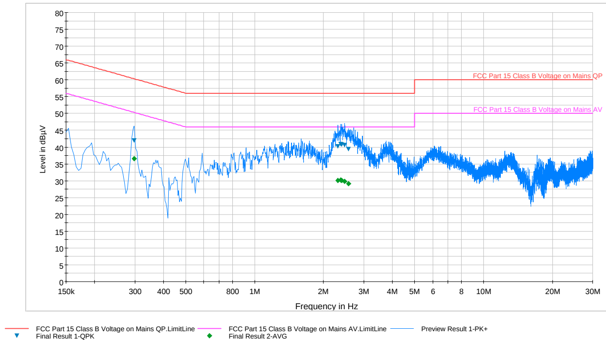
Plot 6-73. Line Conducted Plot with 802.11a UNII Band 3 (N)
