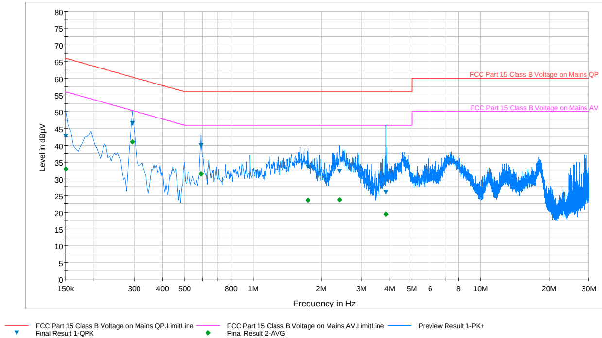
Plot 6-72. Line Conducted Plot with 802.11a UNII Band 3 (L1)
