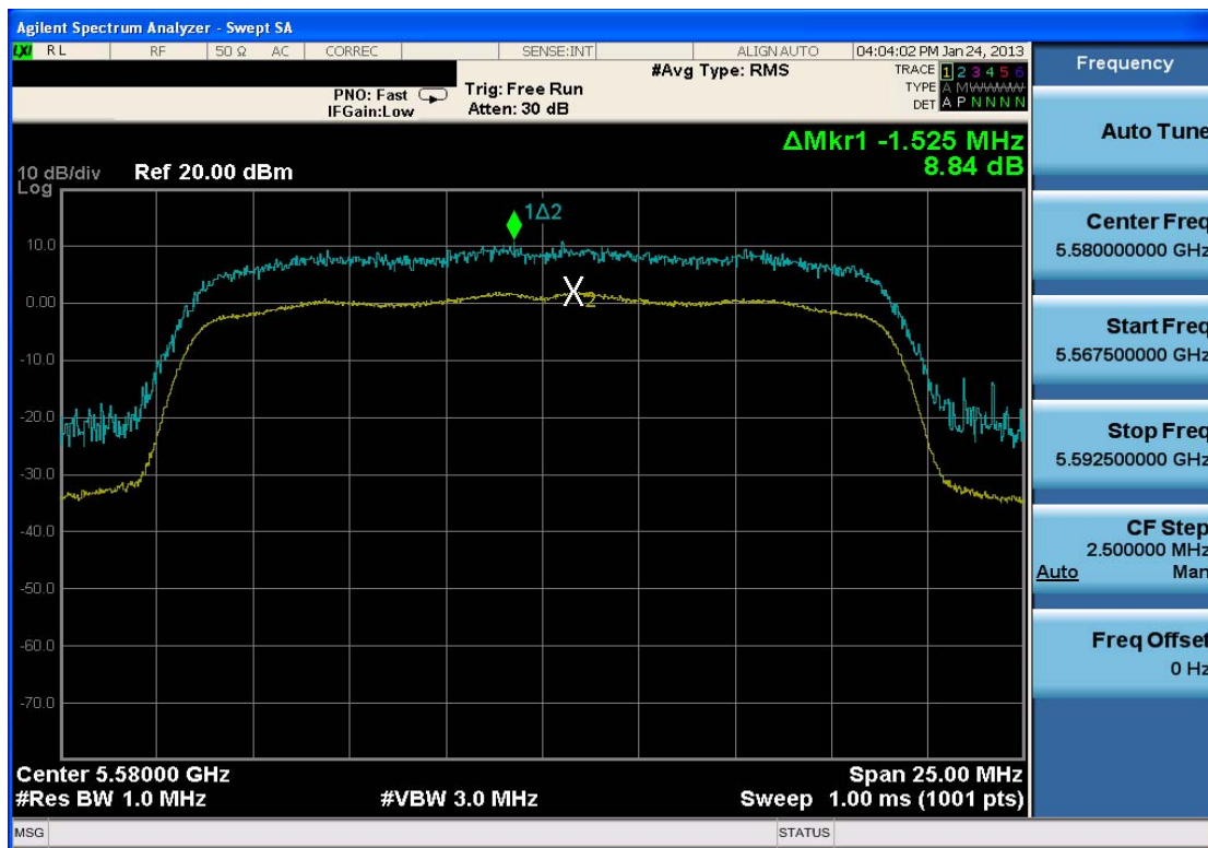
Plot 6-52. Peak Excursion Ratio Plot (20MHz BW 802.11n)
